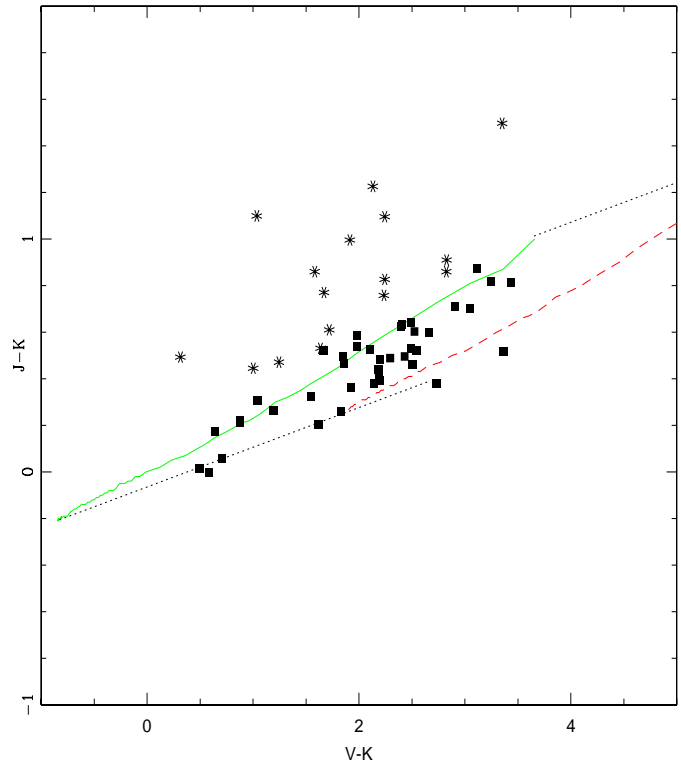
Fig. 6. (J-K)-(V-K) plot for 57 stars in NGC 1893. The lines show the loci of main sequence stars for E(J-K)=0 (solid line) and 0.65 (dashed line). The reddening vectors are indicated by dotted lines. Asterisks indicate objects suspected to be PMS candidates, as discussed in the text
