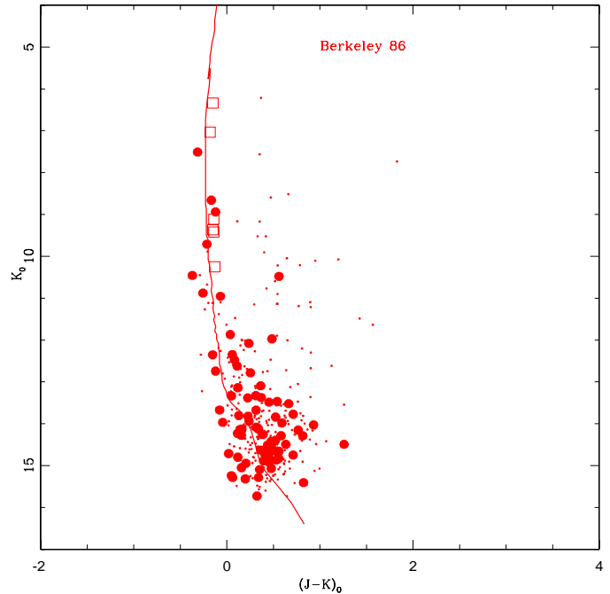
Fig. 10. Reddening corrected CMD of Berkeley 86 with an isochrone from Padova models having an age of 6 Myr. Solid circles indicate suspected members, selected on the basis of the reddening, open squares represent members known from spectroscopy (Massey et al. 1995).
