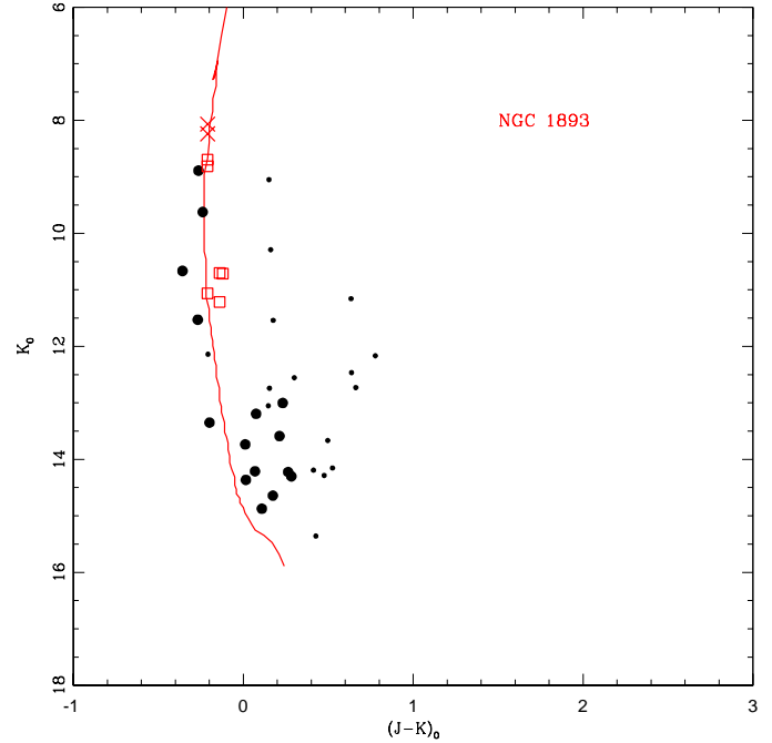
Fig. 4. De-reddened CMD for 38 stars in the field of NGC 1893, obtained as described in the text. An isochrone from Padova models having an age of 4 Myr is plotted. Solid circles represent candidate members, selected on the basis of the reddening. Open squares indicate bona fide members on the basis of Tapia et al. spectroscopy. Crosses show the bona fide members brighter than K=9 not included in our observed field taken from Tapia et al. photometry.
