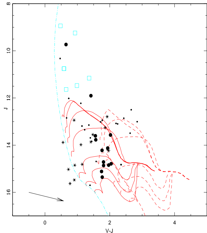
Fig. 8. J-(V-J) plot for 57 stars in NGC 1893. The dashed-dotted lines show 4 Myr isochrones having E(J-K)=0.2 . The lines show the loci of PMS stars by Bernasconi (1996) having E(J-K)=0.2 (solid line) and 0.4 (dashed line) and masses 1.5, 1.7, 2, 3, 4, 5, 7 M_{\odot} . Open squares indicates main sequence stars of known membership from spectroscopy. Solid circles are suspected members derived from reddening analysis as described in the text. Asterisks show objects having infrared excess. The arrow indicates the reddening vector corresponding to E(J-K)=0.2 .
