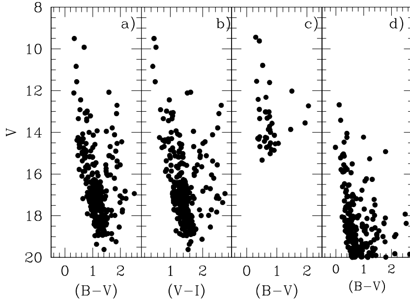
Fig. 4. CMDs of the stars in the region of NGC 133. Panel a) all the stars in the V vs. (B - V) plane. Panel b) all the stars in the V vs. (V - I) plane. Panel c) the CMD by Jasevicius (1964). Panel d) A simulation of the Galactic disk component in the direction of NGC 133.
