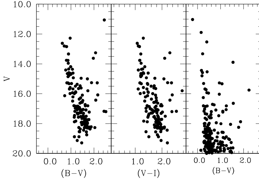
Fig. 10. CMDs of the stars in the region of NGC 1348. Left panel: all the stars in the V vs. (B-V) plane. Central panel: all the stars in the V vs. (V-I) plane. Right panel: a simulation of the Galactic disk component in the direction of NGC 1348.
