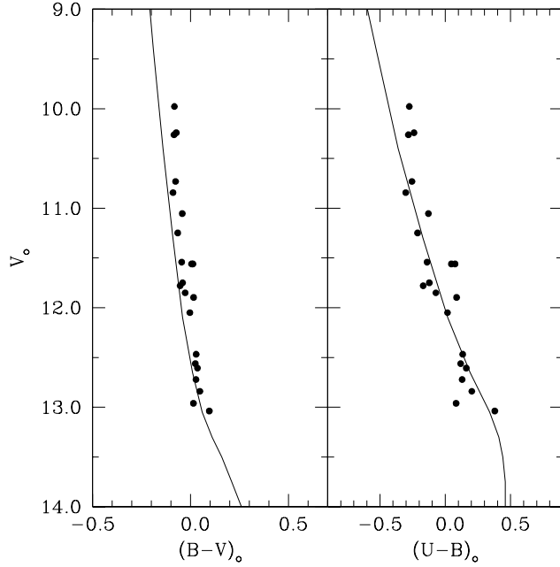
Fig. 13. Reddening corrected CMDs of the likely member stars in the region of NGC 1348.
