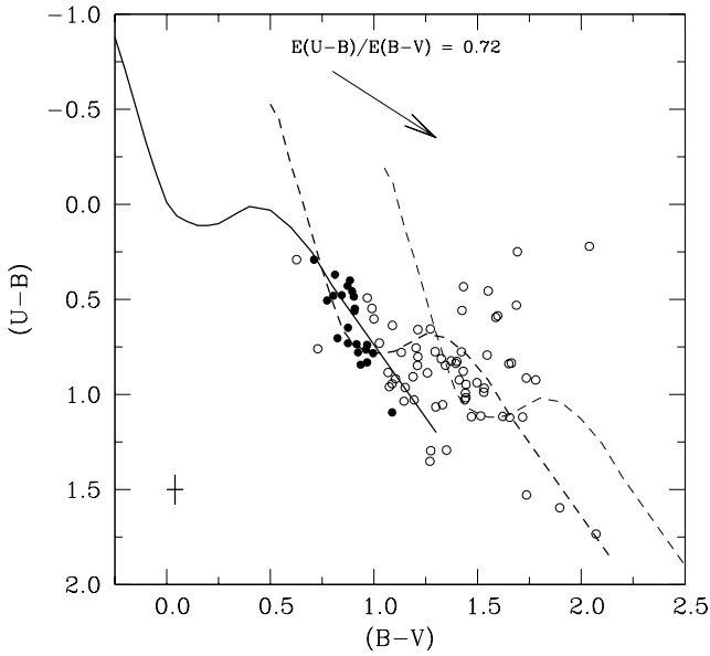
Fig. 11. Color-color diagram for all the stars in the field of NGC 1348 having UBV photometry. The solid line is the Schmidt-Kaler (1982) empirical ZAMS, whereas the dashed and dotted lines are the same ZAMS, but shifted by E(B-V) = 0.85 and 1.5 , respectively. The cross indicates the typical error bars.
