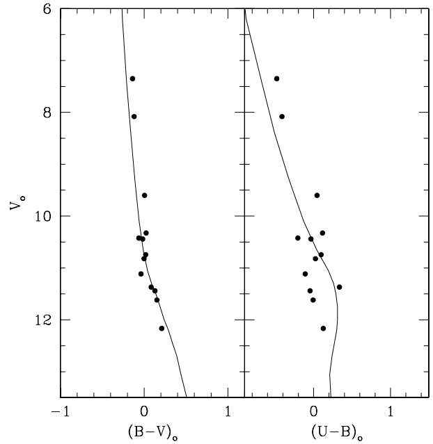
Fig. 7. Reddening corrected CMDs of the likely member stars in the region of NGC 133.
