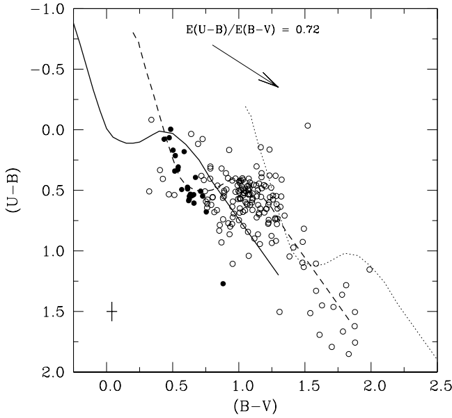
Fig. 5. Color-color diagram for all the stars in the field of NGC 133 having UBV photometry. The solid line is the Schmidt-Kaler (1982) empirical ZAMS, whereas the dashed and dotted lines are the same ZAMS, but shifted by E(B - V) = 0.55 and 1.4 , respectively. The cross indicates the typical error bars.
