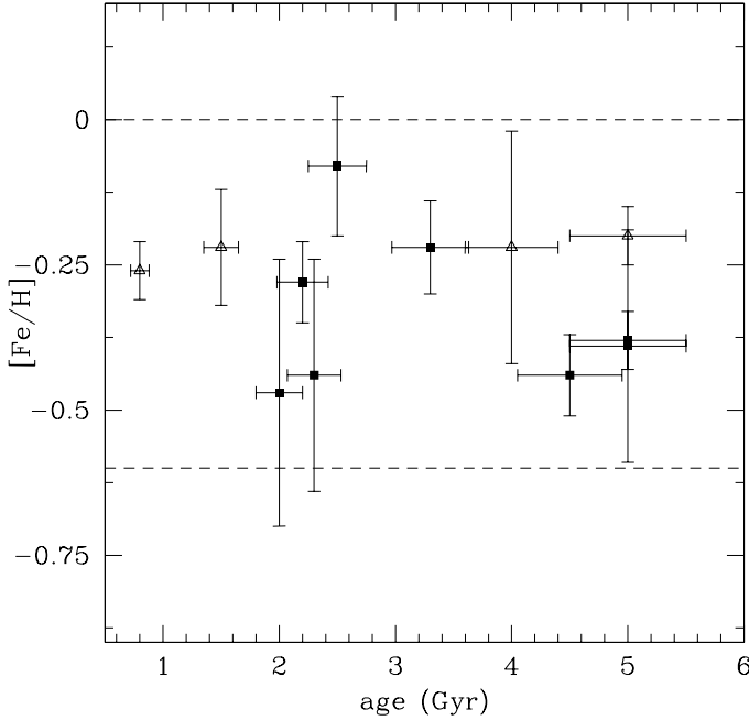
Fig. 4. Age metallicity distribution, with symbols as in Fig. 3. The dashed lines indicate the metallicity range of old open clusters in the Galactic disk, from Friel et al. (2002).
