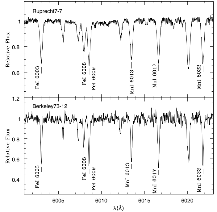
Fig. 1. The spectrum of Ruprecht 7-7 (upper panel) and Berkeley 73-12 (lower panel) in the wave-length interval 6000–6025 Å. Several spectral lines are identified.
