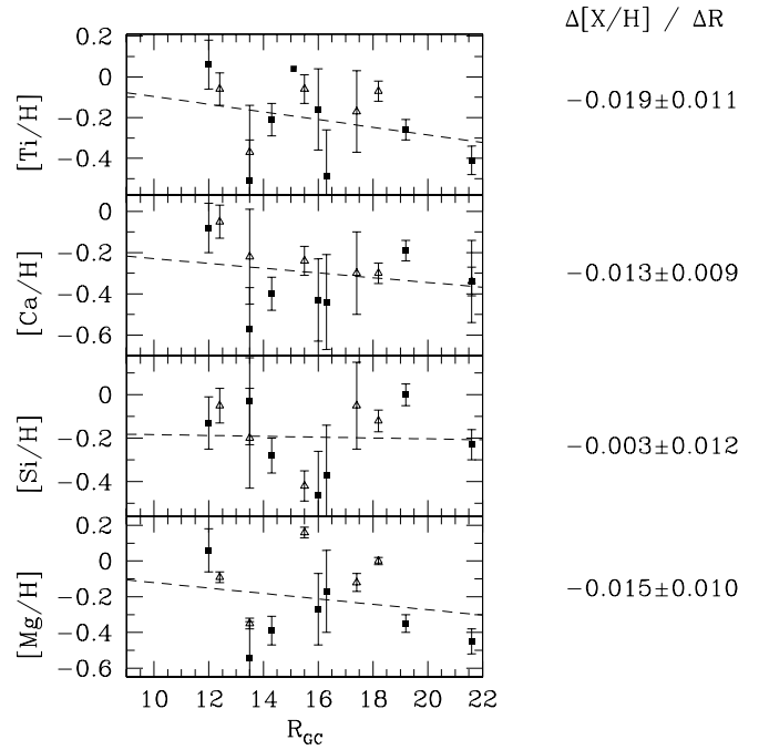
Fig. 6. The radial abundance gradient of Mg, Si, Ca and Ti from old open clusters in the distant Galactic anti-center. The symbols are the same as those used in Fig. 3. On the right the gradient slopes in the range 12 to 22 kpc are indicated.
