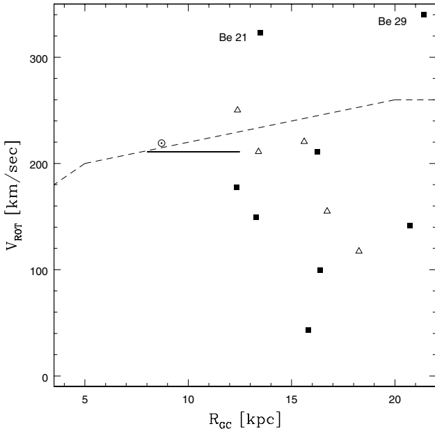
Fig. 8. Rotational velocity of old open clusters in the third Galactic quadrant beyond 12 kpc from the Galactic center. The dashed line is the stellar disk rotation curve from Olling & Merrifield (2000), while the thick solid line is the typical location of old open clusters in the solar vicinity. Symbols are as in Fig. 3.
