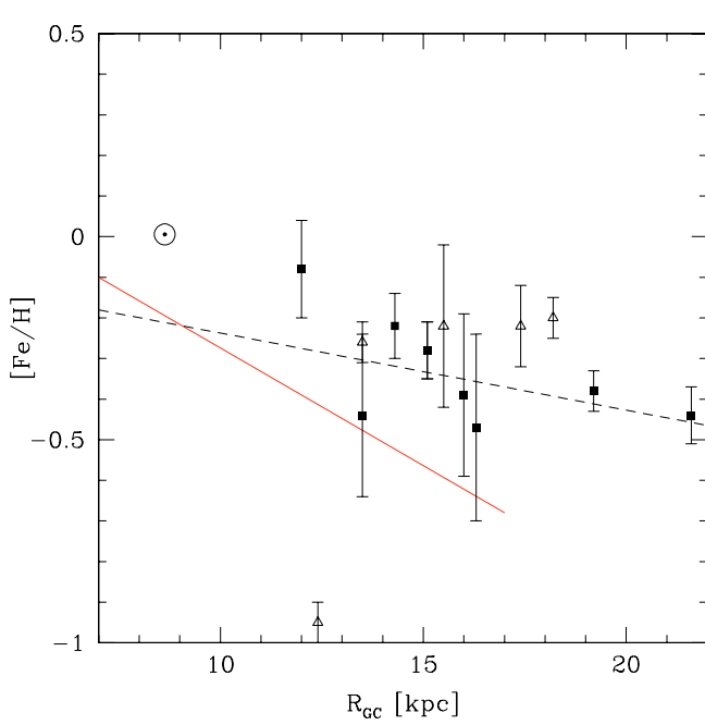
Fig. 5. The radial abundance gradient from old open clusters in the distant anticenter direction. Symbols are as in Fig. 3. The solid line is the Friel et al. (2002) mean abundance gradient, while the dashed line is the gradient when outer disk clusters are added.
