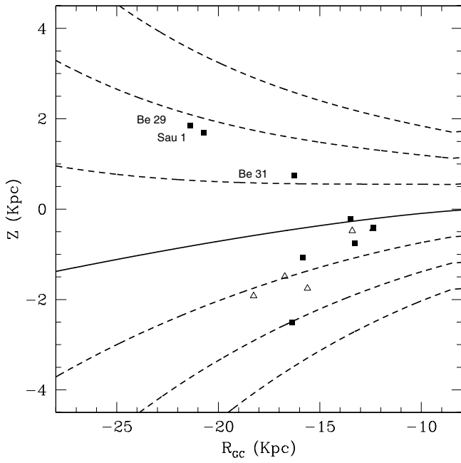
Fig. 7. Distribution of star clusters according to their height above the Galactic plane and distance from the Galactic center. The various lines indicate the warping/flaring of the disk for b = 0^\circ (solid line) and \pm 1, 2 and 3 scale heights (dashed lines). Symbols are as in Fig. 3.
