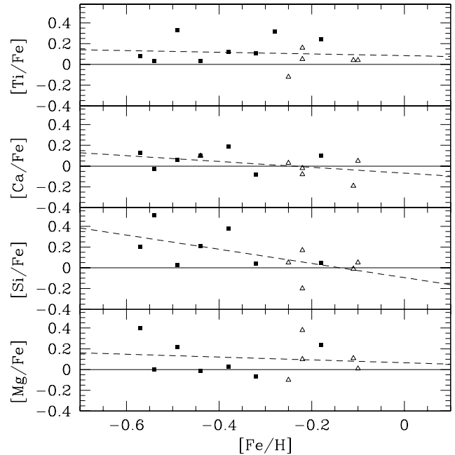
Fig. 3. The trend of \alpha element abundances with metallicity. Open triangles indicate the five program clusters, while filled squares are additional anti-center clusters culled from the literature. The dashed line is a fit through the data.
