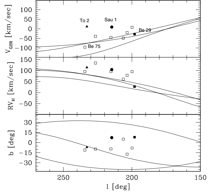
Fig. 9. Location and kinematics of old open clusters in the Galactic anti-center. Superimposed are Peñarrubia et al. (2005) models of the Monoceros Ring. The filled circle indicates Saurer 1, whilst the filled square Berkeley 29 and the filled triangle Tombaugh 2, previously indicated as MRi members.
