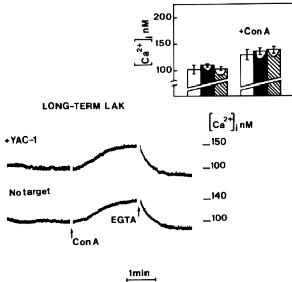
FIGURE 3. Interaction with susceptible targets does not increase [Ca^{2+}]_i in long-term LAK cells. Conditions as in Fig. 1. Where indicated, Con A (10 \mu\text{g/ml} ) and EGTA (1 mM) were added. (Inset) The mean [Ca^{2+}]_i ( \pm SE) at the moment of resuspension (bars on the left) and the maximum rise induced by Con A (bars on the right). LAK cells centrifuged: ( \square ) without targets ( n = 4 ); ( \blacksquare ) with P815 ( n = 3 ); or ( \boxtimes ) YAC-1 cells ( n = 6 ).
