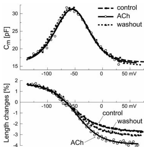
Figure 4. Functional decoupling of electromotility and nonlinear capacitance after ACh application. Capacitance–voltage relationships C_m ( V ) (top) and the voltage dependence of electromotile responses \Delta L ( V ) (bottom), measured before (control; closed squares), during (ACh; open circles), and after (washout; closed triangles) ACh application. Data are from the same experiment shown in Figure 3, A and C–F . Capacitance data were fitted by the scaled derivative of Boltzmann functions with the following parameters: C_{\text{max}} = 15 \text{ pF} , C_0 = 16 \text{ pF} , V_p = -55 \text{ mV} , and W = 21 \text{ mV} (control); C_{\text{max}} = 15 \text{ pF} , C_0 = 16 \text{ pF} , V_p = -50 \text{ mV} , and W = 21 \text{ mV} (ACh); and C_{\text{max}} = 16 \text{ pF} , C_0 = 15 \text{ pF} , V_p = -57 \text{ mV} , and W = 22 \text{ mV} (washout). Motility data were fitted by the Boltzmann functions with the following parameters: \Delta L_{\text{max}} = 4.5\% , V_p = -56 \text{ mV} , and W = 25 \text{ mV} (control); \Delta L_{\text{max}} = 5.6\% , V_p = -52 \text{ mV} , and W = 23 \text{ mV} (ACh); and \Delta L_{\text{max}} = 4.9\% , V_p = -58 \text{ mV} , and W = 24 \text{ mV} (washout).
