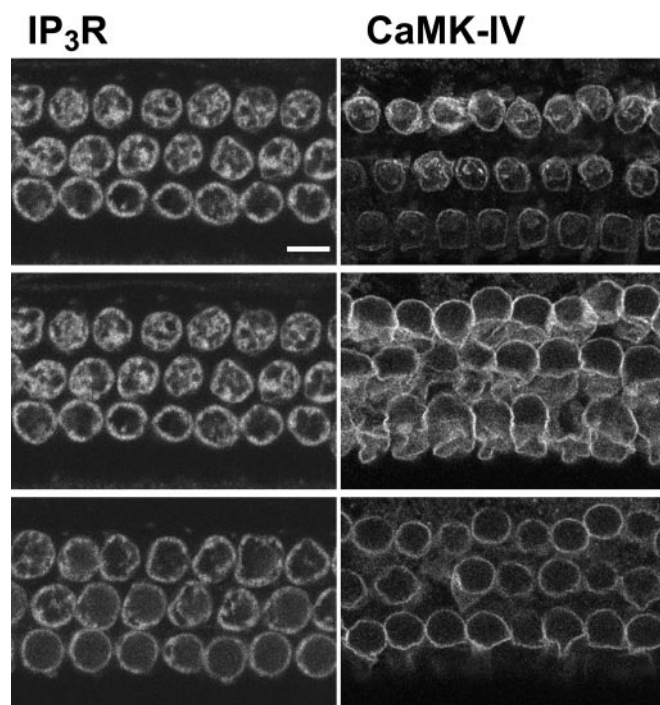
Figure 8. Colocalization of \text{IP}_3 receptors ( \text{IP}_3\text{R} ; left) and \text{CaMK-IV} (right) to the lateral wall of OHCs by confocal immunofluorescence microscopy. Optical cross sections ( 0.4 \mu\text{m} ) were taken at 20 \mu\text{m} intervals, below the cuticular plate (top), halfway down the length of the cells (middle), and in the nuclei region (bottom). In both cases, the antibodies distinctly labeled the lateral wall of the OHC visualized as annular fluorescence patterns. Scale bar, 10 \mu\text{m} .
