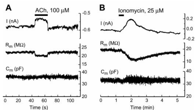
Figure 6. ACh ( A ) and ionomycin ( B ) do not affect the OHC capacitance even under perforated-patch conditions. From top to bottom, the following parameters were measured: I , whole-cell current; R_m , membrane resistance; and C_m , membrane capacitance. The closed horizontal bars at the top of A and B indicate the timing of drug application.
