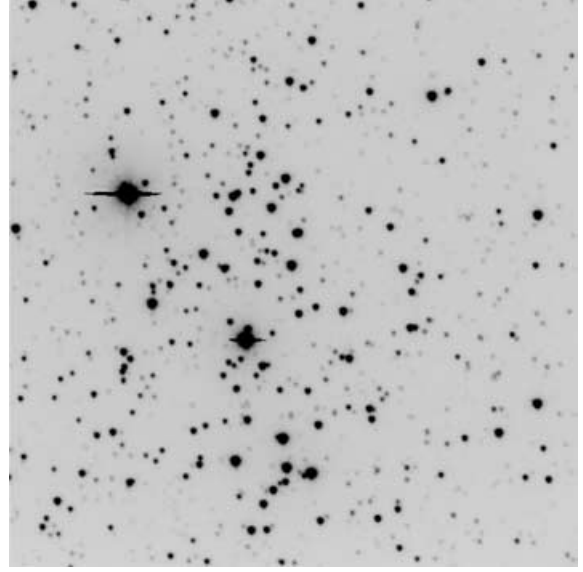
Figure 4. I = 600 s image of Czernik 37. North is up, east on the left and the covered area is 4.1 \times 4.1 arcmin 2 .
