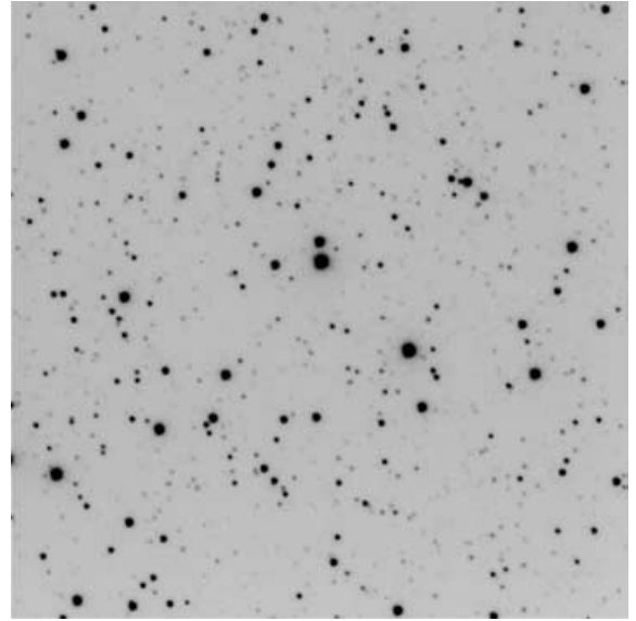
Figure 8. I = 600 s image of King 25. North is up, east on the left and the covered area is 4.1 \times 4.1 arcmin 2 .
