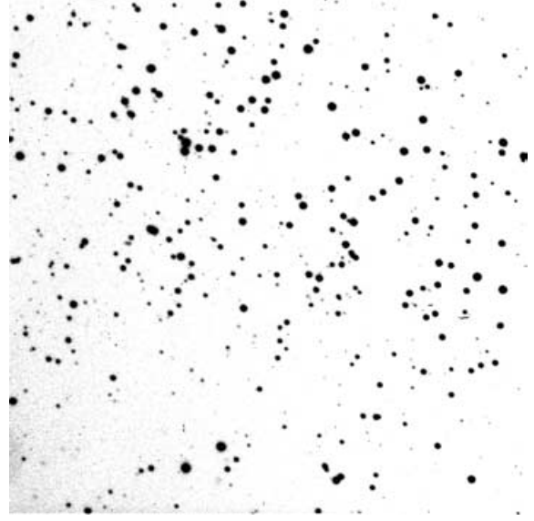
Figure 7. B = 900 s image of Lynga 9. North is up, east on the left and the covered area is 4.1 \times 4.1 arcmin 2 .
