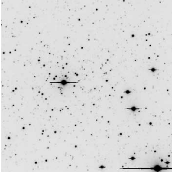
Figure 5. I = 600 s image of BH 150. North is up, east on the left and the covered area is 4.1 \times 4.1 arcmin 2 .
