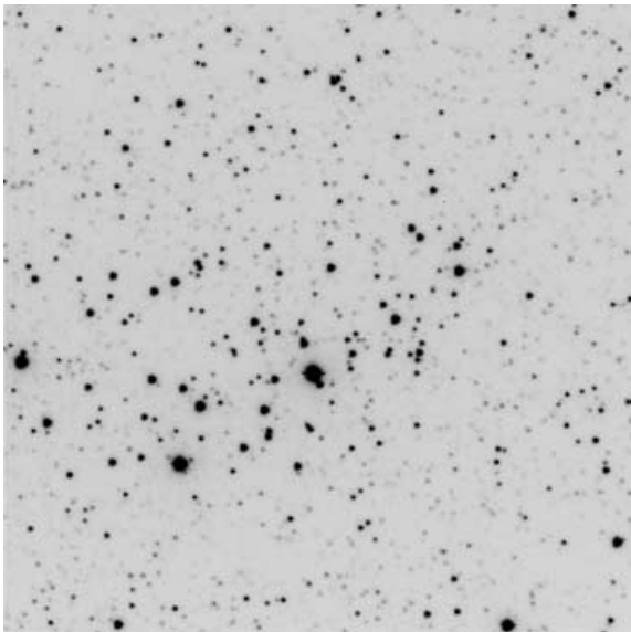
Figure 2. I = 600 s image of Berkeley 80. North is up, east on the left and the covered area is 4.1 \times 4.1 arcmin 2 .
