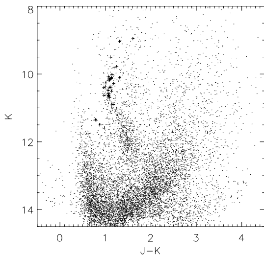
Figure 12. K versus J - K cmd for 2MASS stars within a 10-arcmin field of view around the Lynga 9 position. The plus signs indicate the Lynga 9 ‘clump’ stars from Fig. 11 with V between 14.5 and 16.5 and V - I between 2 and 3.
