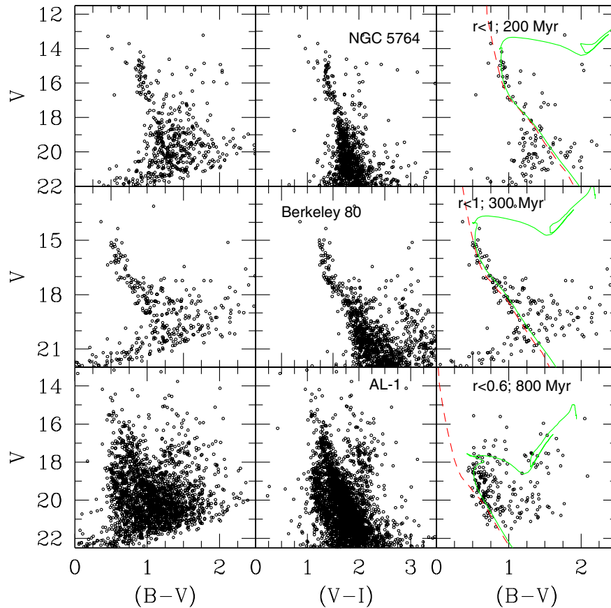
Figure 9. CMDs of the stars in the field of AL 1, Berkeley 80 and NGC 5764. Left panels: all the stars in the V versus (B - V) diagrams. Central panels: all the stars in the V versus (V - I) diagrams. Right panels: Stars lying within r arcmin from the cluster centre (indicated for each cluster). The dashed line is the empirical ZAMS from Schmidt-Kaler (1982), whereas the solid lines are isochrones from Girardi et al. (2000) for the solar metallicity and the indicated age.
