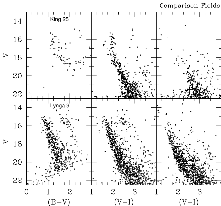
Figure 11. CMDs of the stars in the field of Lynga 9 and King 25 and their offset fields. Left panels: all the cluster stars in the V versus (B - V) diagram. Middle panels: all the cluster stars in the V versus (V - I) diagram. Right panels: all the field stars in the V versus (V - I) diagram.
