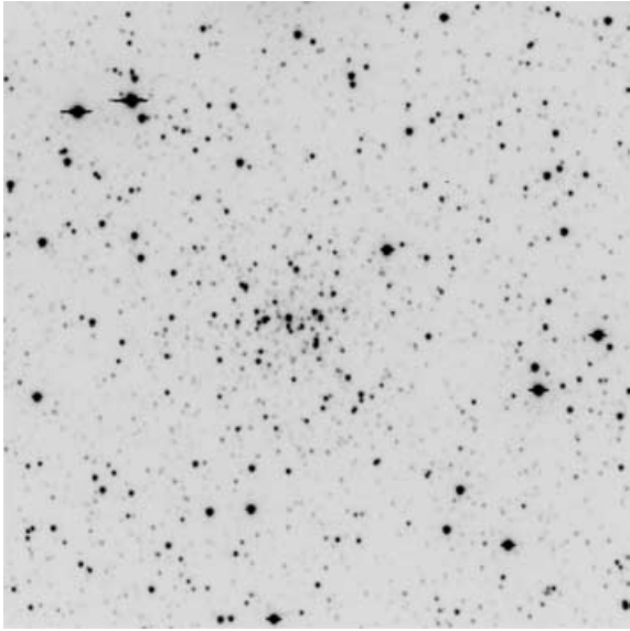
Figure 1. I = 1200 s image of A-L 1. North is up, east on the left and the covered area is 4.1 \times 4.1 arcmin 2 .
