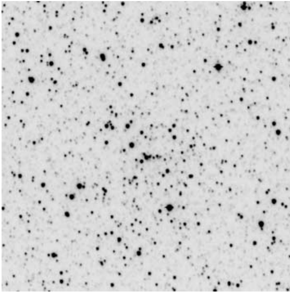
Figure 6. I = 600 s image of BH 261. North is up, east on the left and the covered area is 4.1 \times 4.1 arcmin 2 .
