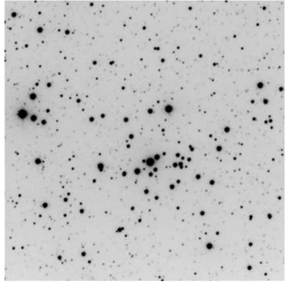
Figure 3. I = 600 s image of NGC 5764. North is up, east on the left and the covered area is 4.1 \times 4.1 arcmin 2 .
