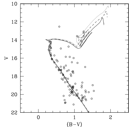
Fig. 13. Three 600 million year isochrones with different metallicities fitted to the sequence of NGC 2635 in the V vs. B - V plane, for a circular extraction of 1.5' . The solid, dashed and dotted lines are Z = 0.019 , Z = 0.008 and Z = 0.004 , respectively.
