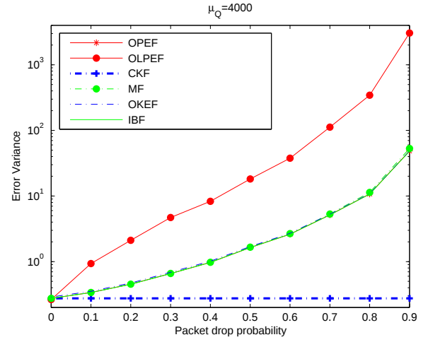
Fig. 4. Error Variance vs. packet drop probability; \mu_Q = 4000 . The curve relative to OPEF is not visible since it coincide, to any practical purpose, with that corresponding to IBF.
