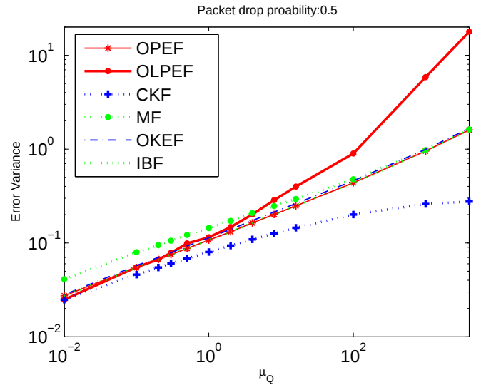
Fig. 1. Error Variance vs. \mu_Q . The curve relative to OPEF coincide, to any practical purpose, with that corresponding to IBF.
