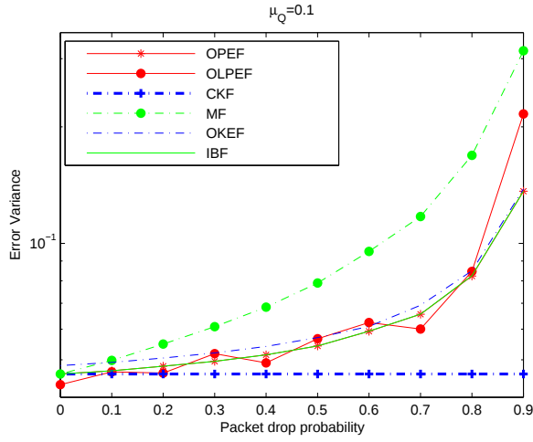
Fig. 2. Error Variance vs. packet drop probability; \mu_Q = 0.1 . The curve relative to OPEF is not visible since it coincide, to any practical purpose, with that corresponding to IBF.
