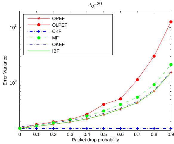
Fig. 3. Error Variance vs. packet drop probability; \mu_Q = 20 . The curve relative to OPEF is not visible since it coincide, to any practical purpose, with that corresponding to IBF.
