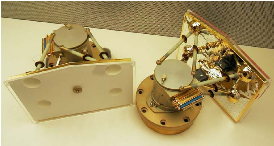
Figure 25. NAC and WAC focal plane assembly.
