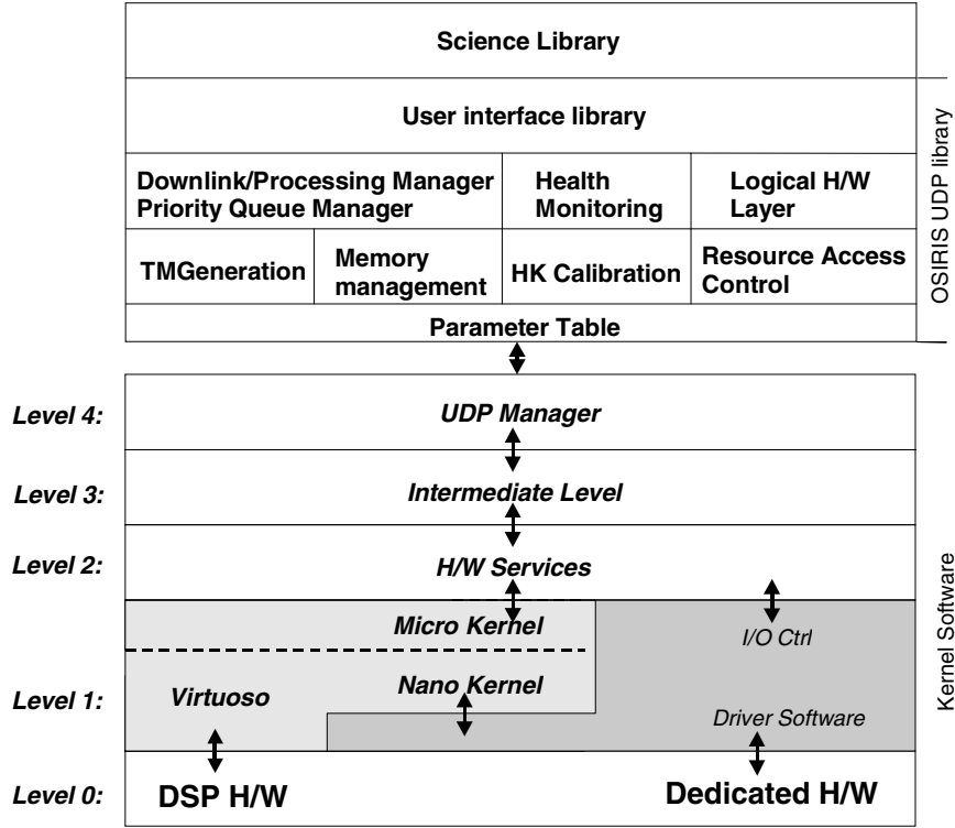
Figure 33. Structure of the OSIRIS flight software.
