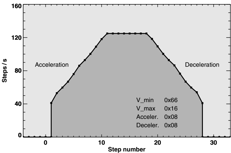
Figure 29. Nominal ramping of the motor step frequency.
