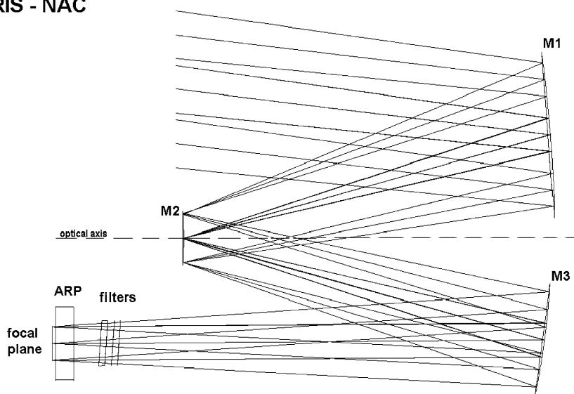
Figure 6. Ray paths through the NAC optical system.
