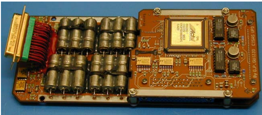
Figure 19. Shutter electronics board.
