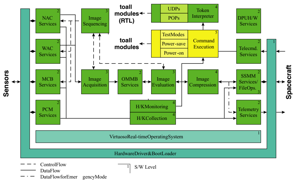
Figure 34. Interaction between software modules within OSIRIS.
