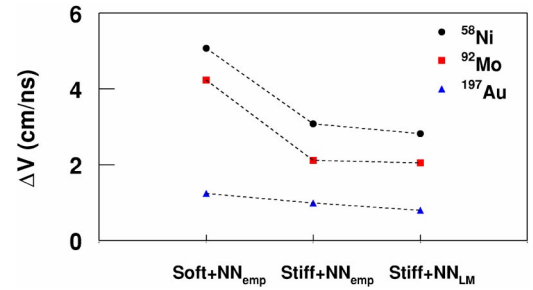
FIG. 3. (Color online) Difference of the peak values of the parallel velocity distribution of nucleons from the projectile and from the target. Peak values are obtained by a Gaussian fit around each peak. Dashed lines are the guide to eye.
