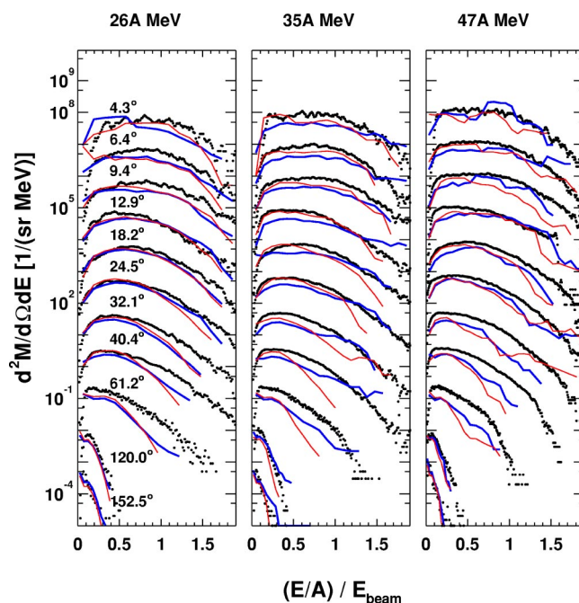
FIG. 22. (Color online) Similar plots to Fig. 19, but for tritons.
