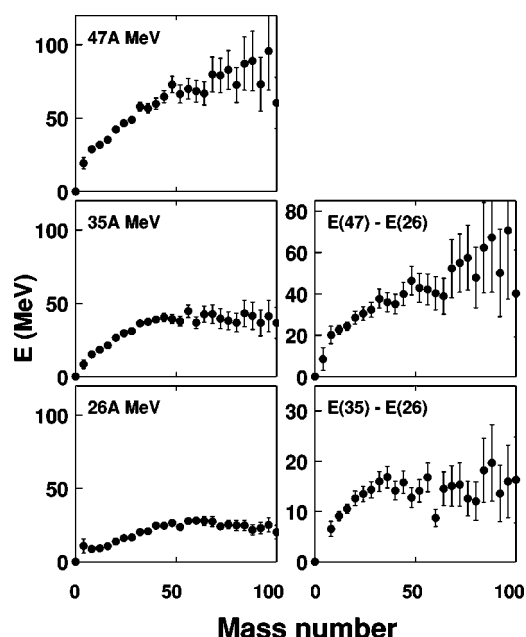
FIG. 39. (Left) Average kinetic energy of fragments in the center of mass system as a function of fragment mass number for ^{197}\text{Au} . Incident energy is indicated in each panel. Energy is evaluated at the time when the fragment is identified at the first time. (Right) Subtracted kinetic energy of fragments for E_k at 47A MeV— E_k at 26A MeV in the upper panel and for E_k at 35A MeV— E_k at 26A MeV in the lower one.
