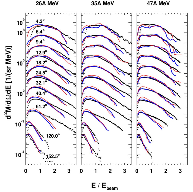
FIG. 19. (Color online) Proton energy spectra for the violent collisions for ^{92}\text{Mo} at three incident energies. The incident energy is indicated at the top of each figure. The spectra in each column correspond to the energy spectra at different angles, indicated in the left column. Experimental results are shown by dots. Thick and thin solid lines correspond to calculated results for Soft+ NN_{emp} and Stiff+ NN_{LM} , respectively. For all cases the differential multiplicity is given in absolute units. In order to avoid the overlap of the data spectra are multiplied by factors of 10^n ( n = 0, 1, 2, 3, 4, 5, 6, 7, 8, 9, 10 ) from bottom to top. No experimental filter is used for the calculated events.
