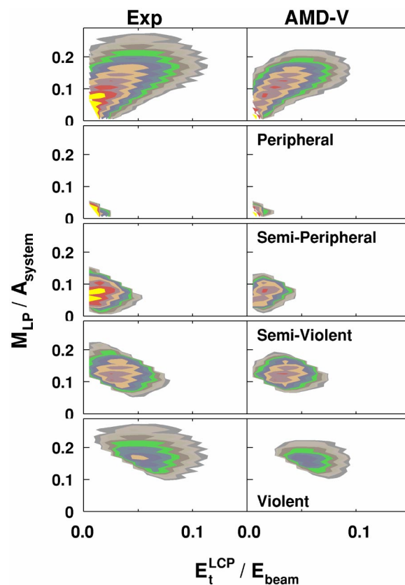
FIG. 8. (Color online) 2D plots of the experimental (right) and the calculated (left) M_{LP}/A_{\text{system}} vs E_t^{LCP}/E_{\text{beam}} for ^{92}\text{Mo} at 47A MeV. M_{LP} is the observed multiplicity of light particles, including neutrons, and A_{\text{system}} is the total nucleon number of the reaction system. E_t^{LCP} is the sum of transverse energy of the light charged particles with Z \leq 2 and E_{\text{beam}} is the projectile incident energy. Generated events by AMD-V has been filtered through the experimental acceptance. Contours are in logarithmic scale and the scale is set arbitrarily.
