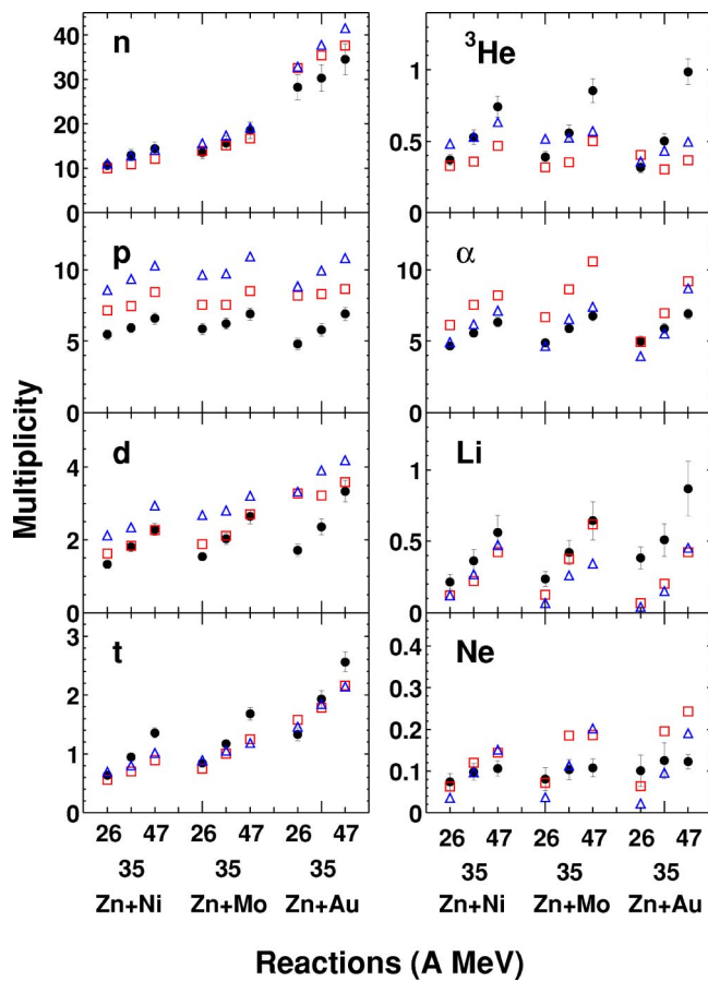
FIG. 15. (Color online) Summary of mean multiplicities of selected particles for the violent class of events for all reactions. Experimental values are efficiency corrected but calculated ones are nonfiltered values. Reaction systems and incident energies are indicated on the x axis and particle is indicated in each panel. Experimental results are shown by solid dots and calculated results with soft EOS+ NN_{emp} and stiff EOS+ NN_{LM} are shown by open squares and triangles, respectively.
