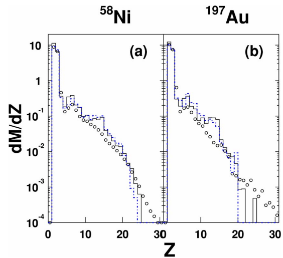
FIG. 17. (Color online) Angle integrated charge distributions of events in violent collisions for (a) ^{58}\text{Ni} and (b) ^{197}\text{Au} at 47 A MeV. Dot-dashed and solid lines correspond to soft EOS+ NN_{emp} and stiff EOS+ NN_{LM} , respectively.
