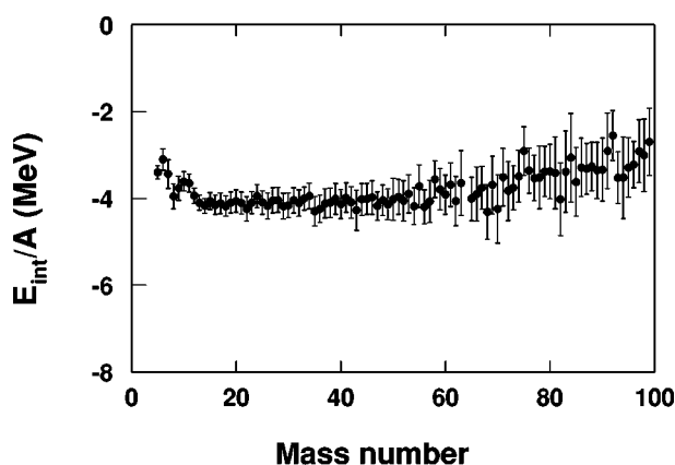
FIG. 38. Average internal energy distribution of fragments with A \geq 5 for ^{197}\text{Au} at 47A MeV. The energy is evaluated when the fragments are identified at the first time.
