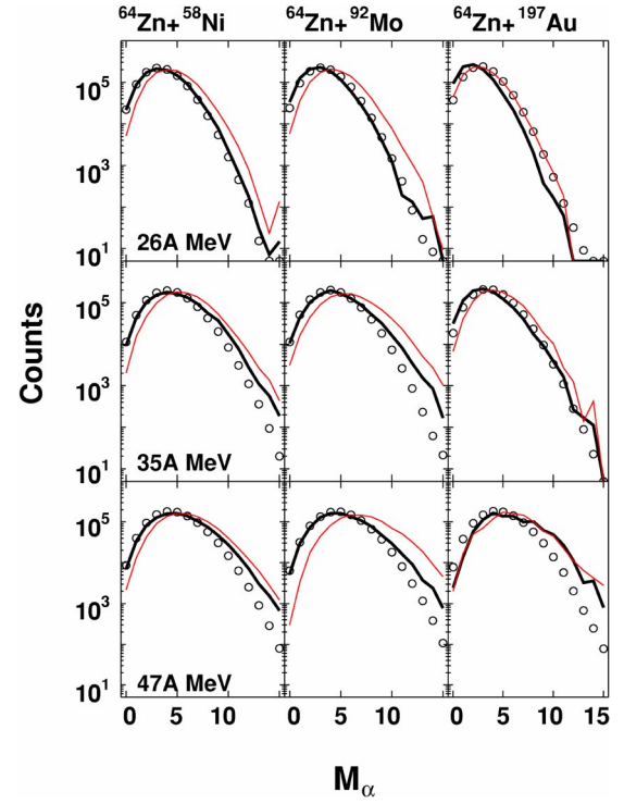
FIG. 14. (Color online) Similar plot to Fig. 13 but for \alpha particles.
