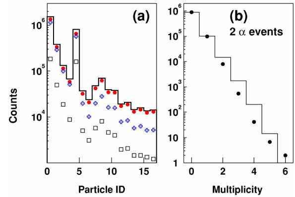
FIG. 6. (Color online) (Left) Number of particles generated by the calculation for {}^{92}\text{Mo} at 47A MeV. Total number of charged particles is given by a histogram as a function of particle ID. The particle ID is given by ID=0, 1, 2, 3, 4 for p , d , t , {}^3\text{He} , \alpha , and ID= Z+2 for Z \geq 3 , respectively. The number of single-hit particles is given by dots and that of double-hit particles is shown by squares. The number of the detected single-hit particle is shown by crosses. (Right) Number of double \alpha hit events is shown as a function of multiplicity for the experiment (dots) and the simulation (histogram). In both cases one million events were analyzed. The calculation is done for the stiff EOS+ NN_{LM} case. The calculated events have been treated by the experimental filter.
