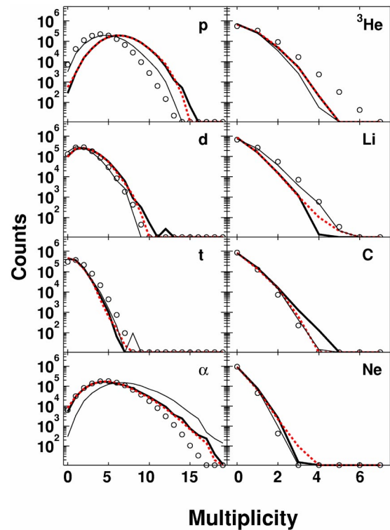
FIG. 12. (Color online) Multiplicity distributions of selected particles for the violent collisions for ^{92}\text{Mo} at 47A MeV. Particles are indicated in each figure. See also the caption of Fig. 11.
