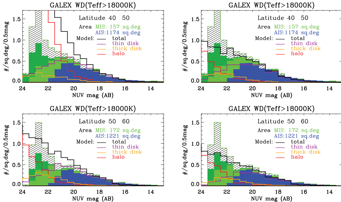
Figure 8. Modelling WD counts: the effect of the IFMR. The density of hot-star candidates at two sample latitudes ( 10^\circ -wide strips) are shown, with model predictions (halo, thin- and thick-disc components, and total) The models in the top-left panel are computed with the TRILEGAL default IFMR (MG07) and the others with W2000 IFMR. The thick disc and halo counts become significant at magnitudes fainter than \sim 19 , and \sim 20 , for these two IFMR, respectively. Models with W2000 IFMR match better the data down to magnitudes \sim 20 – 21 , below which the AIS becomes incomplete. In the top and bottom-right panels the model counts are obtained selecting stars with T_{\text{eff}} > 18000 K in the model calculations, and in the bottom-left panel selecting stars by colour cut ( FUV - NUV < -0.13 ) with TRILEGAL’s transformation from T_{\text{eff}} to magnitudes, from the same calculations. The comparison illustrates the uncertainties introduced by the transformation of the isochrones into magnitudes via model atmospheres. The filled-green histograms are GALEX MIS hot ‘single’ sources with SDSS match (light green), and including sources with no SDSS detection (dark green).
