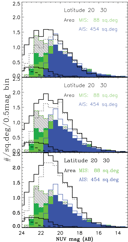
Figure 12. Thin-disc description. In view of the fact that our present data are most sensitive to the thin-disc population, we compare model results computed with three different thin-disc geometries: in the top panel the TRILEGAL default geometry, in the middle panel an exponential (option 1) and in the bottom panel a z sech (option 2) description (see text). The top panel, with the default geometry description given in equations (1) and (2), gives the closest results to the observed counts, confirming previous findings by Girardi et al. (2005). This option was adopted in all our model calculations shown. Colours and symbols as in Fig. 10.
