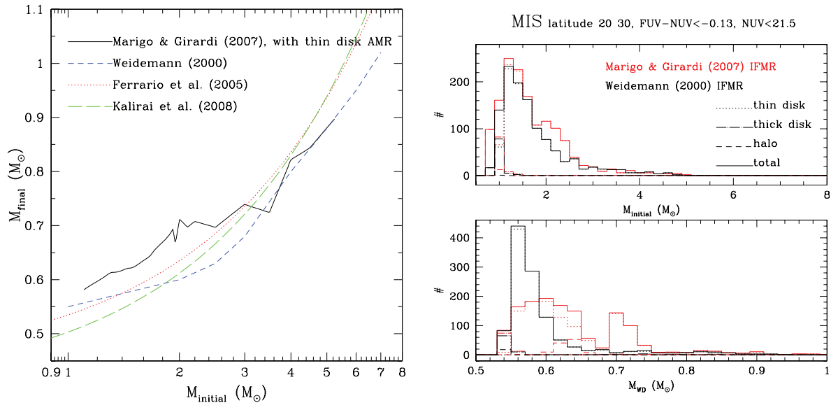
Figure 9. Left: some of the IFMRs implemented in TRILEGAL, and tested in this work. The MG07 IFMR depends on metallicity, so that different age-metallicity relations (AMR) will sample it in different ways; the curve shown here is for the Rocha-Pinto et al. (2000) AMR, which is used to model the MW thin disc in TRILEGAL. Other IFMRs are the semi-empirical one from W2000, and the purely empirical ones by Ferrario et al. (2005) and Kalirai et al. (2008). Right: the distribution of initial and final WD masses (top and bottom panels, respectively) derived from TRILEGAL models using the MG07 (red lines) and W2000 (black lines) IFMR. The different lines illustrate the contributions from the different MW components, for one sample latitude, down to \text{NUV} = 21.5 .
