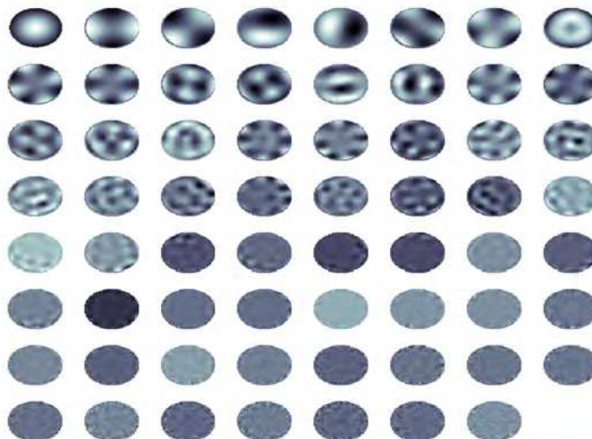
Fig. 9. Modes relative to a 61 electrode membrane DM.
