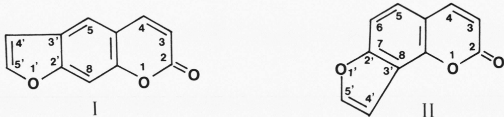
Fig. 1. Molecular structure of psoralen I and angelicin II.
