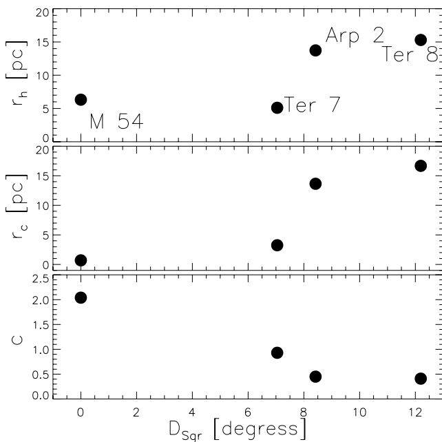
Figure 6. Concentration – distance and core/half radius – distance relations for the bona fide Sgr clusters. M54 is placed at the centre of Sgr (but see Siegel et al. 2011). The data for M54 and Terzan 7 come from Harris (1996), while those for Arp 2 and Terzan 8 come from our measurements.
