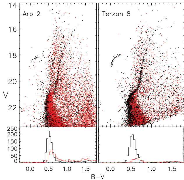
Figure 5. CMD of stars inside (black) and outside (red) the measured tidal radius in Arp 2 and Terzan 8. The lower panels indicate the colour distribution of both populations between V = 22 and 22.5 .
