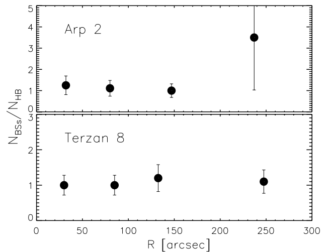
Figure 9. BS specific frequency profiles in Arp 2 and Terzan 8.
