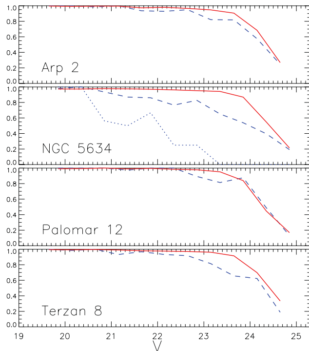
Figure 2. Level of completeness for the V photometry in each cluster. Stars were counted in 0.5 mag bins. The dashed blue line indicates the completeness inside the inner 2 arcmin of each cluster, while the red solid line indicates the completeness outside this radius. NGC 5634 is divided into three bins with 30 \text{ arcsec} < R < 60 \text{ arcsec} (dotted line), 60 \text{ arcsec} < R < 120 \text{ arcsec} (dashed line) and R > 120 \text{ arcsec} (solid line).
