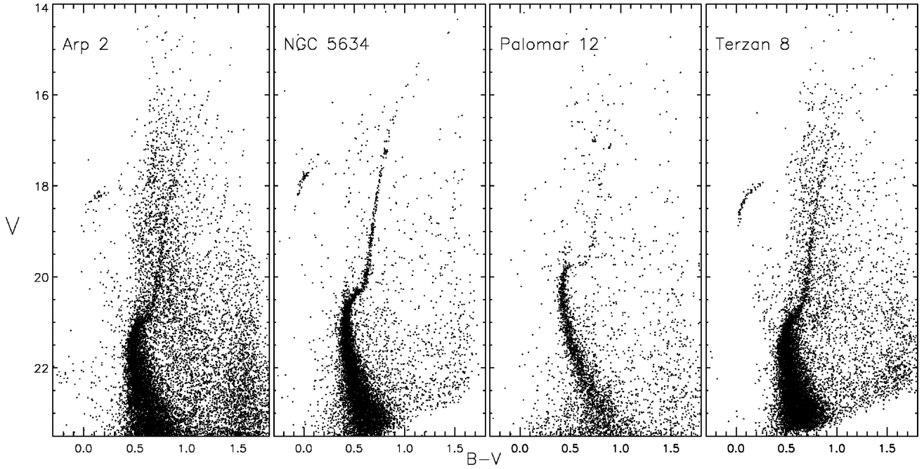
Figure 3. CMDs of the four clusters. Field contamination can be seen as most severe in the case of Arp 2.
