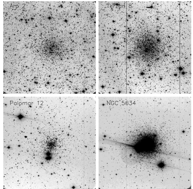
Figure 1. Mediated images produced with MONTAGE2. These images are used to establish the initial positions of the stars that are introduced to ALLFRAME. All images have approximately 14 \times 14 arcmin 2 . North is up and east is to the left.
