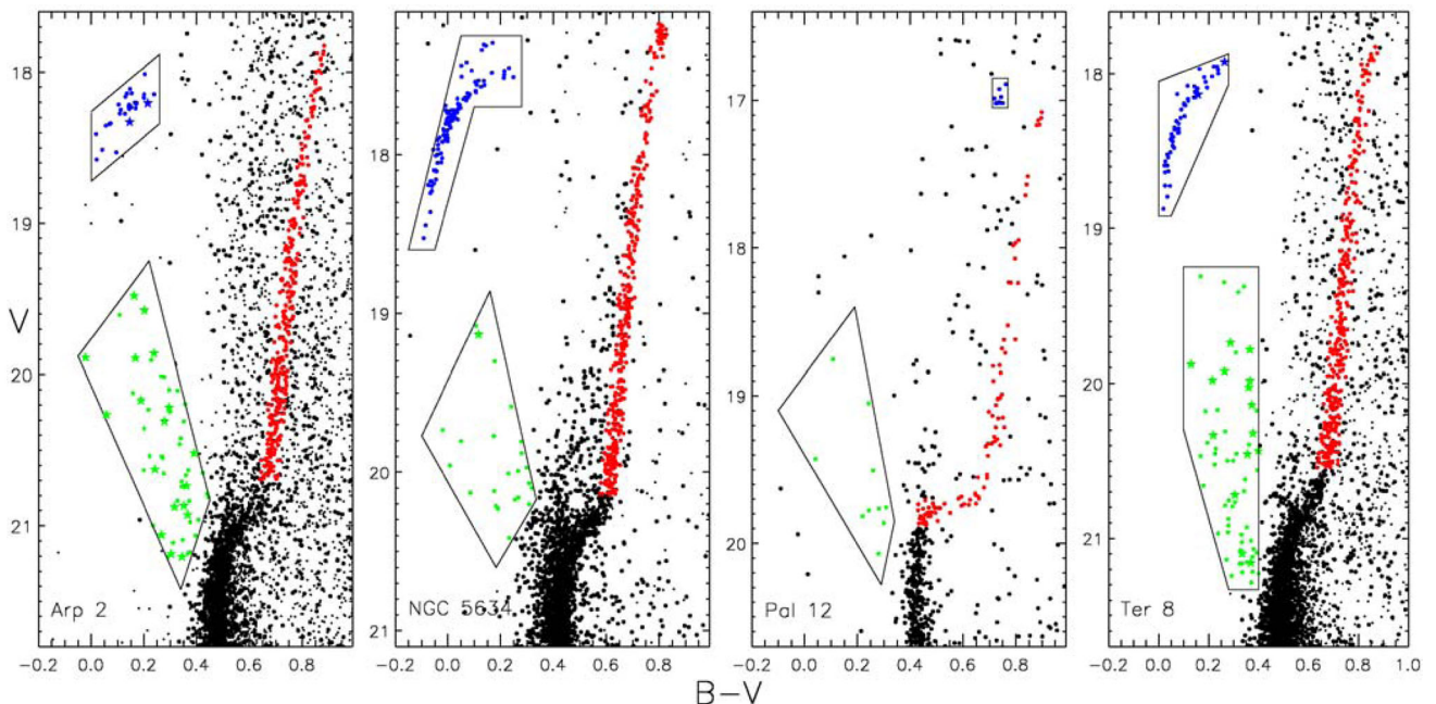
Figure 7. Subpopulation selection criteria. BSs are marked with green symbols, RGB stars with red symbols and HB stars with blue symbols. The starry symbols in the BS and HB regions indicate stars outside the tidal radius of the cluster.
