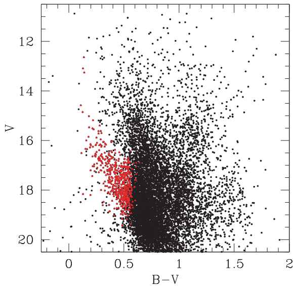
Figure 6. The CMD in the B - V versus V plane of all stars having photometric errors smaller than 0.1 in the direction of the CMa overdensity. With filled triangles (red when printed in colour), we indicate stars belonging to the BPs, as selected in the B - R versus B CMD.
