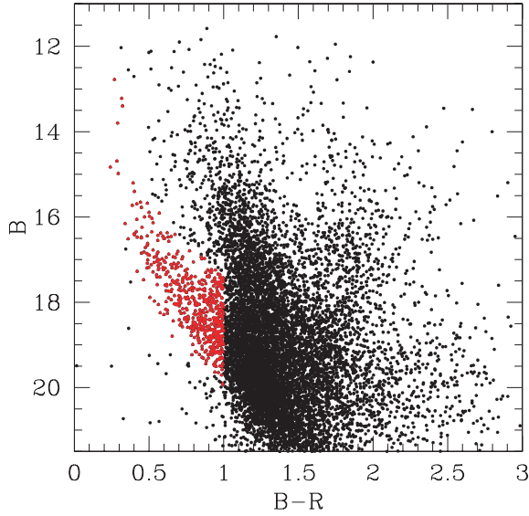
Figure 5. The CMD in the B - R versus B plane of all stars having photometric errors smaller than 0.1 in the direction of the CMa overdensity.
