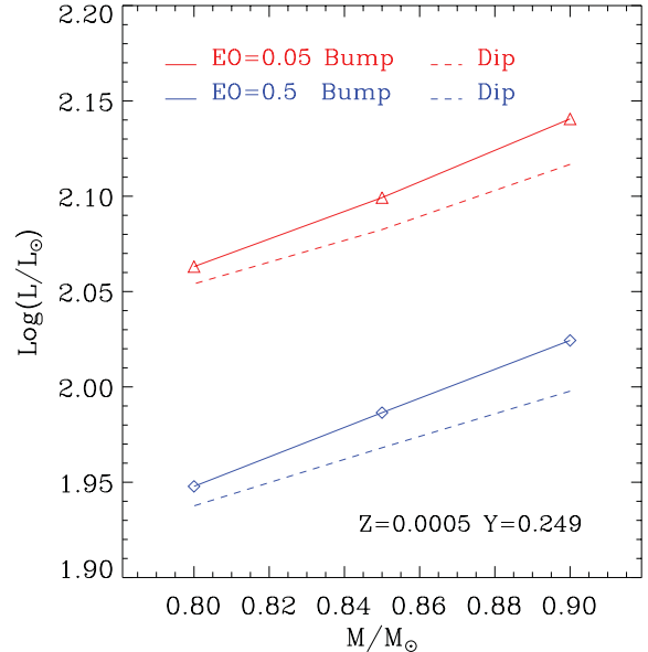
Figure 4. The luminosity both at the maximum (solid lines) and minimum ('dip', dashed lines) of the bump feature along the first-ascendant RGB for a few low-mass tracks of Z = 0.0005 , Y = 0.249 computed with \Lambda_e = 0.05 H_p (red) and \Lambda_e = 0.5 H_p (blue). In models with high \Lambda_e , the RGB bump is typically \sim 0.3 mag fainter than in the model with negligible envelope overshooting.
