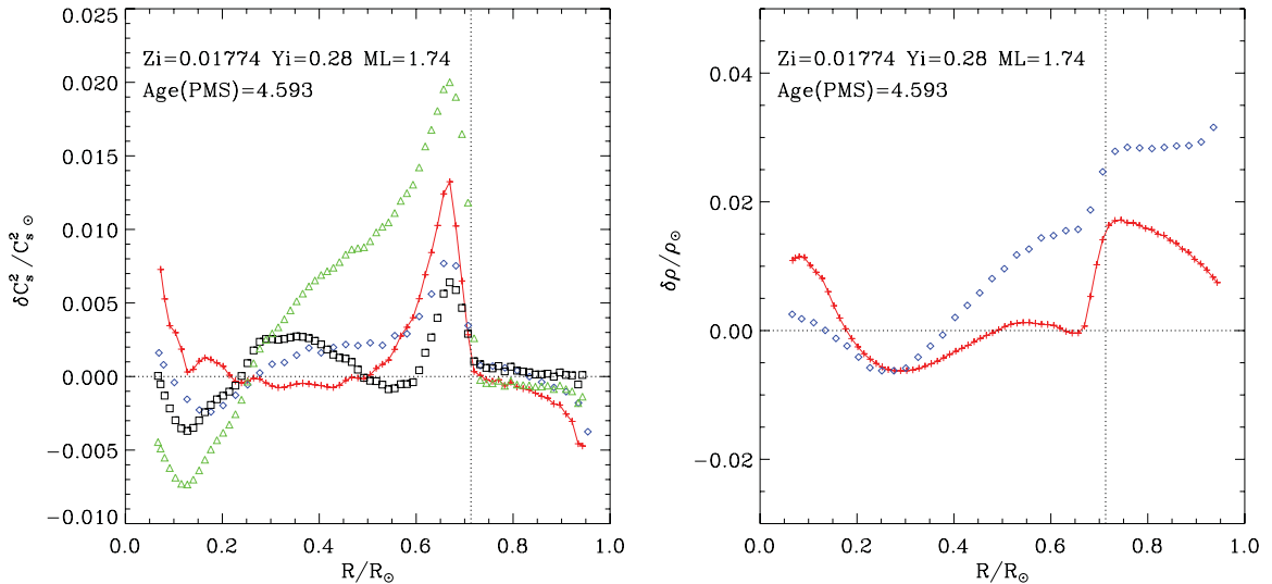
Figure 7. Solar model obtained using the tabulated FREEEOS. Left-hand panel: interior relative differences (in the sense Sun minus model) in the squared sound speed \delta c_s^2/c_s^2 . Solar values are obtained from MDI data (Basu, Pinsonneault & Bahcall 2000). Symbols are as follows. Red crosses: our model; blue diamonds: Basu et al. (2009) model differences with respect to MDI data using Grevesse & Sauval (1998) solar abundances; black squares: Serenelli et al. (2009) using Grevesse & Sauval (1998) solar abundances; green triangles: Serenelli et al. (2009) solar abundances. Right-hand panel: interior relative differences for the density profile. In this case, only the Basu et al. (2009) model is shown for comparison. Z_i , Y_i and ML refer to the initial metallicity and helium abundance and to the \alpha_{\text{MLT}} of our model, respectively. The quoted age includes the PMS lifetime which is about 40 Myr, determined by the stage on the ZAMS where the total gravitational luminosity falls, and remains, below a few per cent. Values obtained from this calibration are shown in Table 3.
