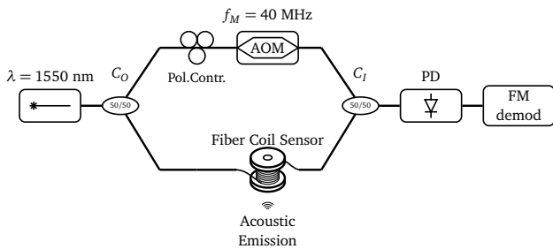
FIG. 2 Setup of the sensing scheme for FCS: the light source is a high-coherence DFB laser at 1550 nm; AOM: acousto-optic modulator at 40 MHz; Co and C1: optical coupler; PD: photodiode; FM demod: double balanced quadrature FM detector board.
