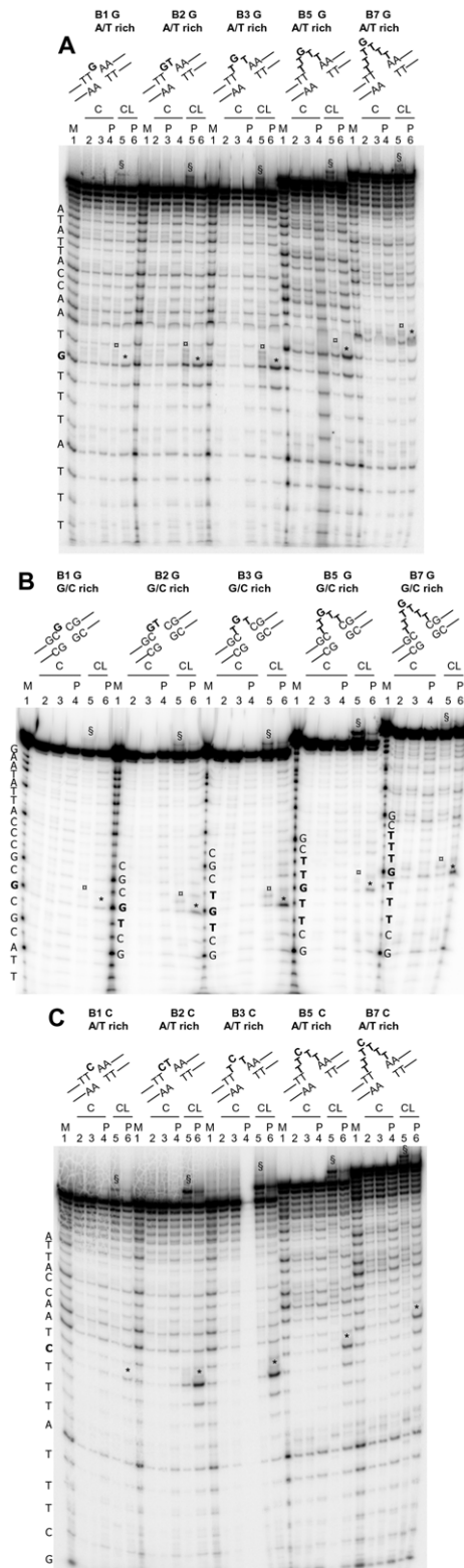
Figure 4. CL footprinting of bulged oligonucleotides. A) Oligonucleotides 1, 6 and 7 were heat denaturated and folded in the presence of the appropriate complementary sequences (1b rev, 1c rev, 1d rev, Table 1) to obtain the bulged G A/T rich oligonucleotides shown above the gel. B) Oligonucleotides 8, 9, 10, 11 and 12 were heat denaturated and folded in the presence of the appropriate complementary sequences (8 rev, 9 rev, 10 rev, Table 1) to the bulged G G/C rich oligonucleotides shown above the gel. C) Oligonucleotides 5, 1, 13,
