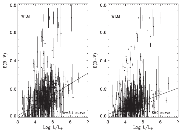
Figure 6. Reddening of WLM stars, derived from multi-band SED fitting using the Galactic (left panel) or the SMC (right panel) extinction curves.
