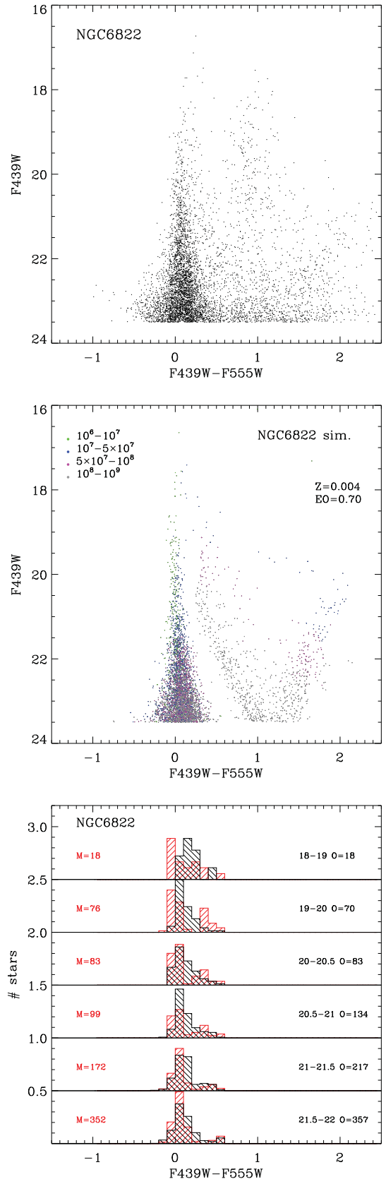
Figure 10. Upper panel: Observed CMD for NGC 6822. Middle panel: The best model obtained with PARSEC V1.1. Lower panel: Comparison of the observed and modelled colour distributions.
