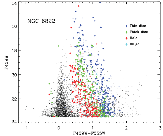
Figure 7. Estimated MW contamination in the CMD of NGC 6822. Black dots are the observed stars while coloured dots are the predicted contamination by the four Galactic components as indicated in the labels.
