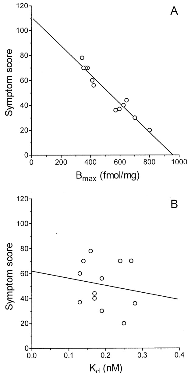
Figure 2. Linear correlation analysis between B_{\max} (A) or K_d (B) values of [ 3 H]paroxetine binding to platelet SERT and symptom score values in D-IBS patients at baseline.
