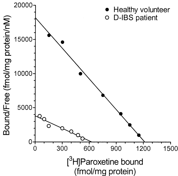
Figure 1. Representative Scatchard plots obtained for binding assay of [ 3 H]paroxetine to platelet SERT of patient 3 and healthy volunteer 2.
