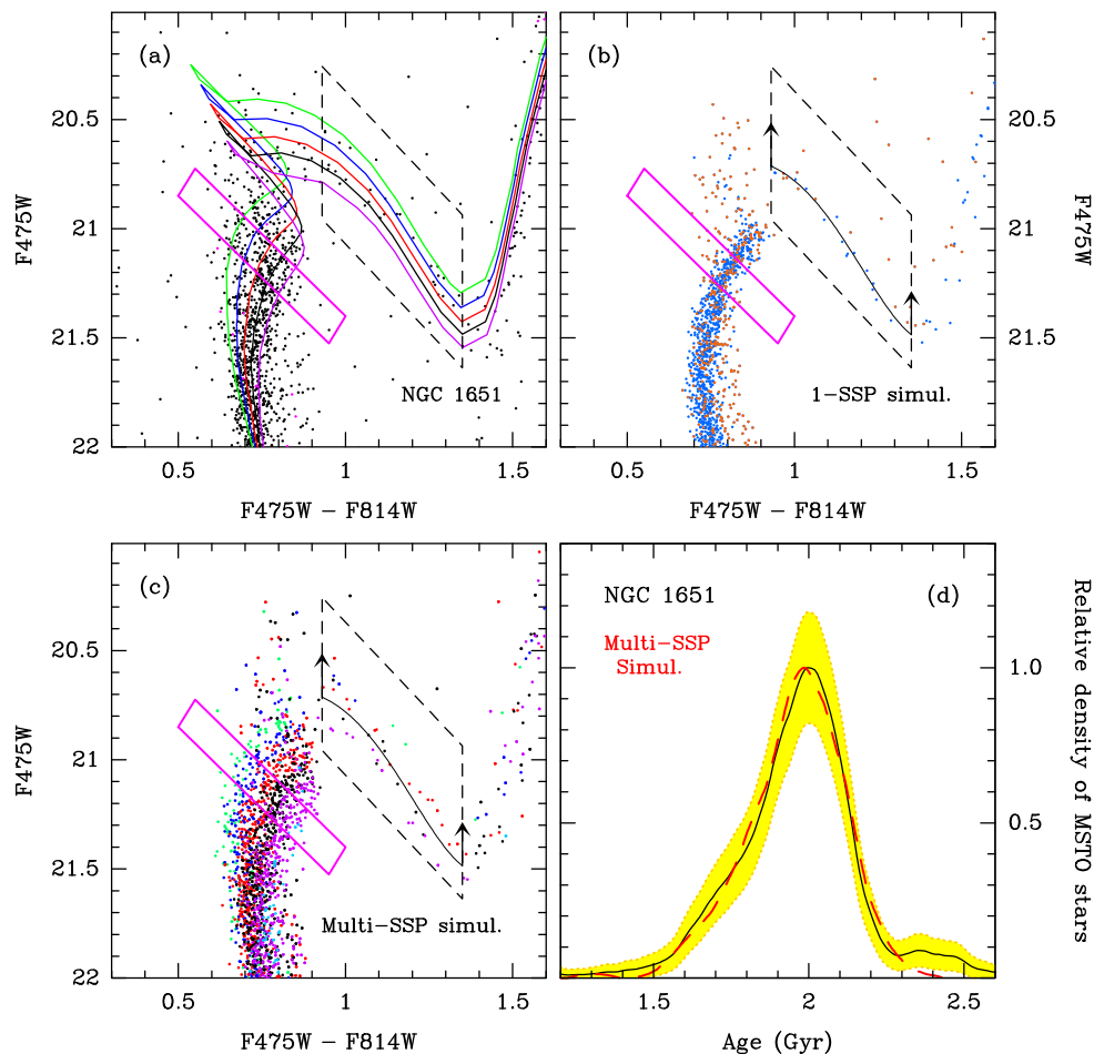
Figure 2. Panel (a): the CMD of NGC 1651 in the MSTO-SGB region (taken from G+14) along with M+08 isochrones for Z = 0.008 and ages 1.7, 1.8, 1.9, 2.0, and 2.1 Gyr. Black dots represent stars within the effective radius of NGC 1651. Red dots indicate stars in the outskirts of the HST image with a total area equal to that within the effective radius of NGC 1651. The SGB selection box is outlined by black dashed lines. For reference, the MSTO crosscut parallelogram used by G+14 to measure the pseudo-age distribution of NGC 1651 is shown in magenta. Panel (b): CMD of a single-SSP simulation of NGC 1651 using the 2.0 Gyr isochrone (see Section 3.1). Single stars are shown as blue dots while unresolved binaries are shown as orange dots. The black solid line within the SGB selection box in panel (b) represents the SGB portion of the isochrone for the best-fitting (mean) age. The black arrows in panel (b) indicate the direction of the positive X axis in the cross-SGB profiles shown in Figs 3–7. Panel (c): similar to panel (b) except that the dots now represent a ‘multi-SSP’ simulation of NGC 1651, described in Section 3.1. Simulated stars with ages of 1.7, 1.8, 1.9, 2.0, 2.1, and 2.2 Gyr are shown in green, blue, red, black, purple, and cyan, respectively. Panel (d): the black solid line represents the pseudo-age distribution of NGC 1651 as measured from the MSTO crosscut by G+14 (cf. Fig. 1a), expressed as a normalized density function, while the yellow region indicates its 68 per cent confidence interval. For comparison, the red dashed line represents the corresponding pseudo-age distribution of the ‘multi-SSP’ simulation described in Section 3.1 for NGC 1651.
