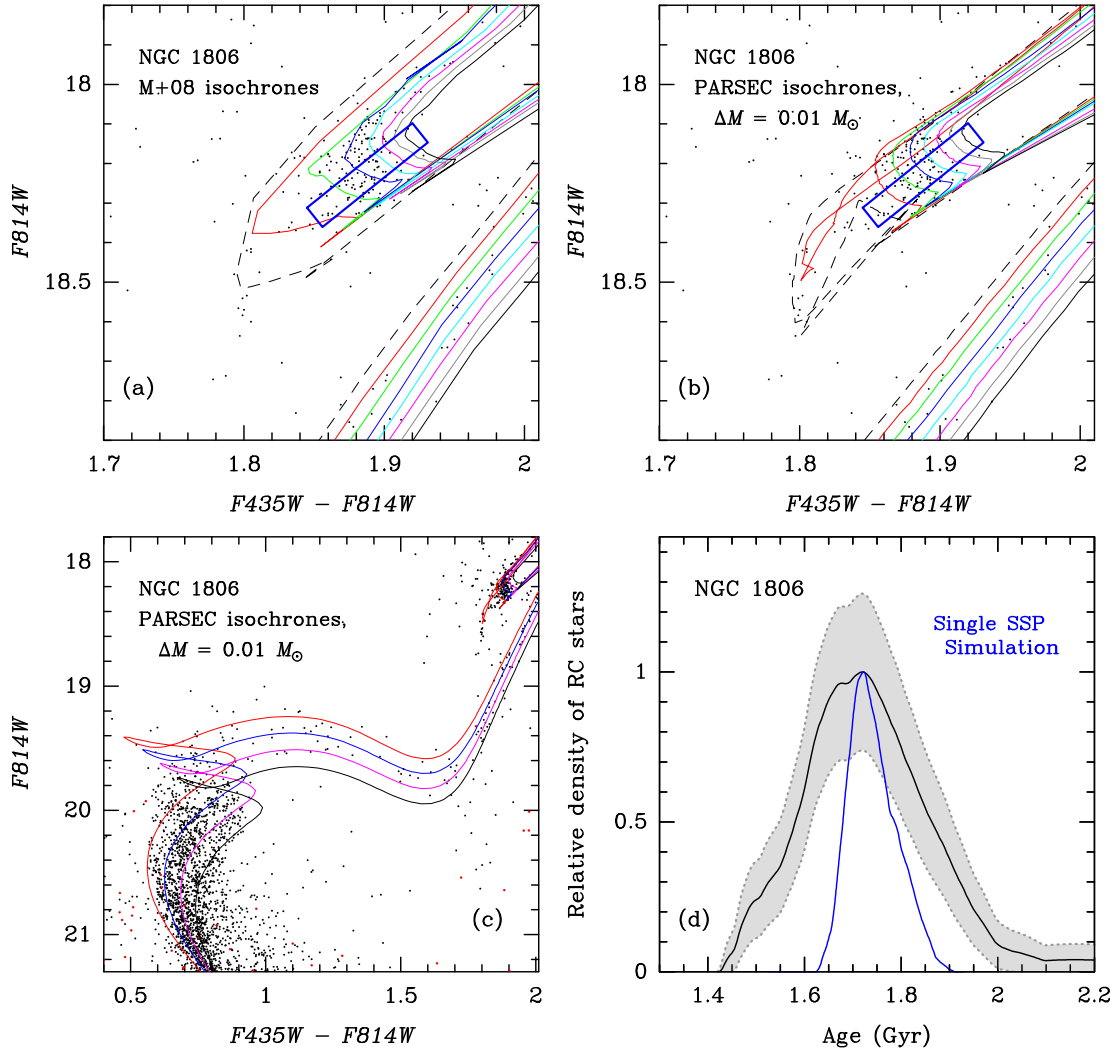
Figure 9. Panel (a): the CMD of NGC 1806 (cf. Fig. 6 a), zoomed in on the RC region. The lines represent M+08 isochrones for \log(\text{age}/\text{yr}) = 9.10 to 9.24 (left to right) with a spacing of 0.02 . Panel (b): same as panel (a), but the lines now represent new PARSEC isochrones with Z = 0.008 which were derived from stellar tracks spaced by \Delta M/M_{\odot} = 0.01 (see Section 4.2). Isochrones are for \log(\text{age}/\text{yr}) = 9.18 – 9.32 (left to right) with a spacing of 0.02 . The thick blue rectangle in panels (a) and (b) is used to derive the age distribution of RC stars as described in Section 4.2. Panel (c): CMD of NGC 1806 showing the region from below the MSTO to beyond the RC along with new PARSEC isochrones for Z = 0.008 and ages of 1.58 , 1.74 , 1.91 , and 2.09 Gyr (left to right). Panel (d): the black solid line shows the cross-RC distribution of NGC 1806 expressed in age units (see Section 4.2), while the light grey region indicates its 68 per cent confidence interval. For comparison, the solid blue line represents the cross-RC distribution of a single-SSP simulation of NGC 1806, divided by a factor \simeq 1.9 to yield the same maximum star density as that of NGC 1806 itself.
