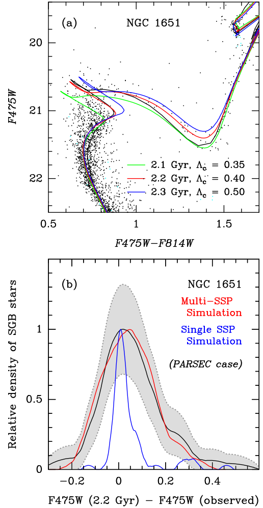
Figure 8. Panel (a): CMD of NGC 1651 showing the upper MS, MSTO, SGB, lower RGB, and RC features. The black line represents the best-fitting M+08 isochrone (cf. Fig. 2 a). The green, red, and blue lines represent PARSEC isochrones with [M/H] = -0.40 for which the ages and overshoot values are indicated in the legend. Panel (b): same as Fig. 3, but now using the SGB of the PARSEC isochrone with age = 2.2 Gyr and \Lambda_c = 0.40 as the zero-point of the cross-SGB profiles. Note the similarity of the cross-SGB profiles of NGC 1651 (black line with 68 per cent confidence interval in light grey) and that of its ‘multi-SSP simulation’ (red line), while the cross-SGB profile of the ‘single-SSP simulation’ (blue line) is much narrower.
