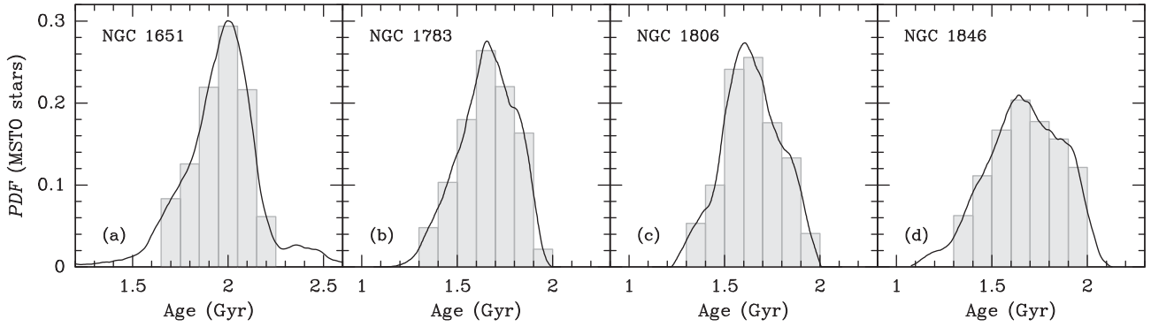
Figure 1. Illustration of the assignment of relative masses to individual SSP ages (i.e. isochrones) for the ‘multi-SSP’ simulations of the four star clusters in our sample that feature eMSTOs (see Section 3.1). Panel (a): the black solid line represents the pseudo-age distribution of NGC 1651 taken from G+14 , expressed as probability density function. The histogram in light grey shows the relative weights of the different age bins used during the simulations. Panel (b): same as Panel (a), but now for NGC 1783, using its pseudo-age distribution taken from G+11a , using ages from the M+08 isochrones. Panel (c): same as Panel (b), but now for NGC 1806. Panel (d): same as Panel (b), but now for NGC 1846, using its pseudo-age distribution taken from Goudfrooij et al. (2009) .
