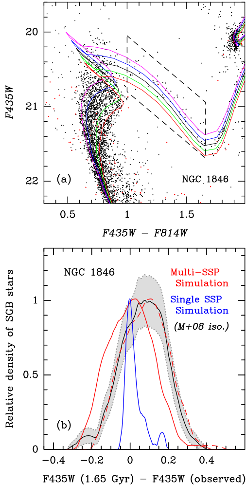
Figure 7. Similar to Fig. 5, but now for NGC 1846. The SGB profile of the ‘Single SSP Simulation’ in panel (b) was divided by a factor of \simeq 4.4 in order to scale its maximum density to that of NGC 1846.
