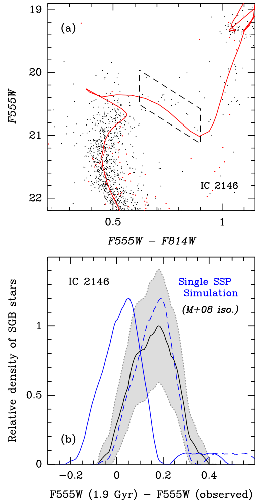
Figure 4. Panel (a): CMD of IC 2146 within its core radius, taken from Correnti et al. (2014), along with an M+08 isochrone of age 1.90 Gyr. The SGB selection box is outlined by black dashed lines. Red dots indicate stars in the outskirts of the HST image with a total area equal to that within the core radius of IC 2146. Panel (b): The black solid line represents the cross-SGB profile for IC 2146, while the light grey region indicates its 68 per cent confidence interval. For comparison, the solid blue line represents the cross-SGB profile of a single-SSP simulation of IC 2146. The blue dashed line is the same after shifting it by 0.13 mag to the right.
