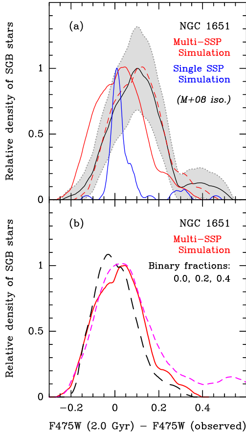
Figure 3. Panel (a): the black solid line represents the cross-SGB profile for NGC 1651, while the light grey region indicates its 68 per cent confidence interval. The red solid line represents the cross-SGB profile of the ‘multi-SSP’ simulation described in Section 3.2.1. The red dashed line is the same after shifting it by 0.08 mag to the right. For comparison, the solid blue line represents the cross-SGB profile of a single-SSP simulation of NGC 1651, divided by a factor of \simeq 3.5 in order to scale its maximum density to that of NGC 1651. Panel (b): Comparison between ‘multi-SSP’ simulations of NGC 1651 created with binary fractions 0.0 (long dashed line), 0.2 (solid line), and 0.4 (short dashed line).
