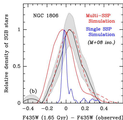
Figure 6. Similar to Fig. 5, but now for NGC 1806. The SGB profile of the ‘Single SSP Simulation’ in panel (b) was divided by a factor of \simeq 4.6 in order to scale its maximum density to that of NGC 1806.
