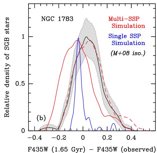
Figure 5. Panel (a): CMD of NGC 1783 within its core radius, taken from G+11a , along with M+08 isochrones of age 1.50, 1.60, 1.70, 1.80, and 1.90 Gyr (top to bottom). Red dots indicate stars in the outskirts of the HST image with a total area equal to that within the core radius of NGC 1783. The SGB selection box is outlined by black dashed lines. Panel (b): similar to Fig. 3, but now for NGC 1783. The SGB profile of the ‘Single SSP Simulation’ was divided by a factor of \simeq 4.5 in order to scale its maximum density to that of NGC 1783.
