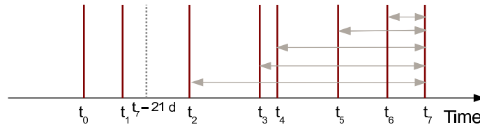
Figure 5. Schematic of the time-clustering algorithm. For an IceCube event in an on-source bin detected at time t_7 the significances of all clusters formed with events detected up to 21 days back are calculated.
