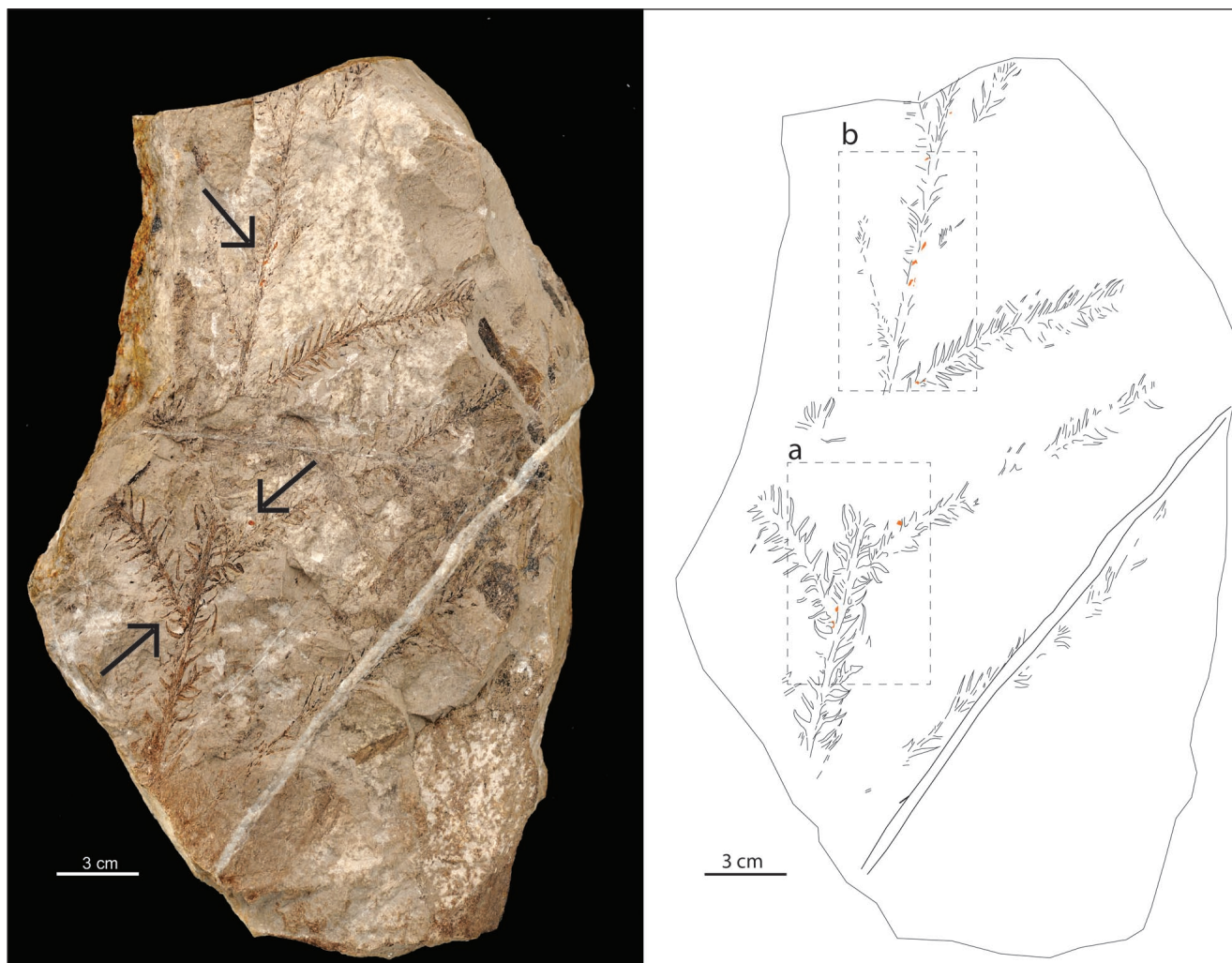
Fig. 4 - Amber and plant remains from the Vienna specimen of Voltzia ladunica NHM 2007B0004-0001; a and b in the drawn plant represent areas shown in detail in Fig. 5a and 5c, respectively.
