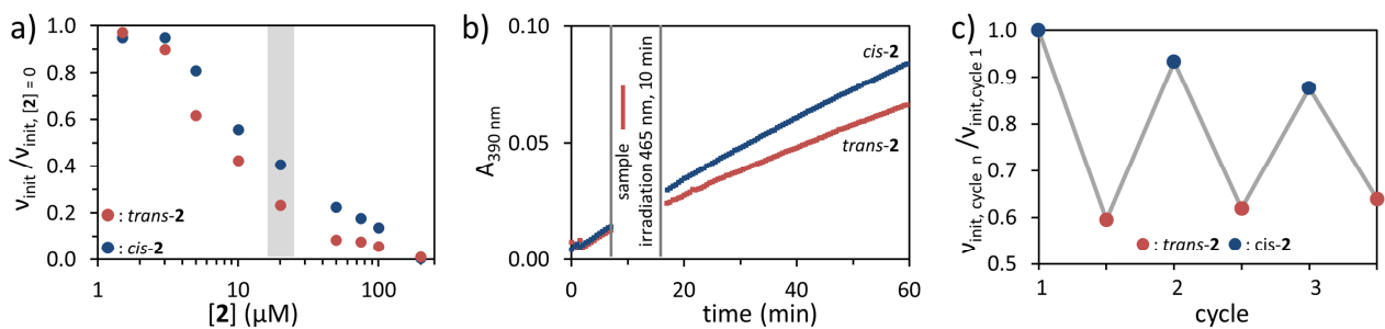
Figure 3. a) Plot of the initial rate (normalized on the rate for [2] = 0 \mu\text{M} ) of the transphosphorylation of HPNPP as a function of the concentrations of cis - and trans - 2 . b) Increase in absorbance as a function of time for samples that were (blue) and were not (red) irradiated at 465 nm for 10 minutes after 7 minutes of reaction. c) Plot of the initial rates (normalized on the initial rate of the first kinetics) for several irradiation cycles. Protocols and experimental conditions are given in the Supporting Information.
