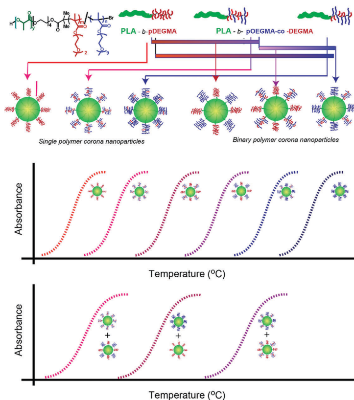
Fig. 1 Structure of polymers and cartoon representation of different PLA-(OEGMA) copolymers used to form thermoresponsive nanoparticles. Individual polymers with varying ratios of (OEG) 3 MA and DEGMA were formed into nanoparticles (“Single polymer corona nanoparticles”) or mixtures of co-polymers were prepared prior to nanoparticle formation (“binary polymer corona nanoparticles”). The resulting nanoparticles displayed variable aggregation temperatures dependent on the relative concentrations of the copolymers in the blends.
