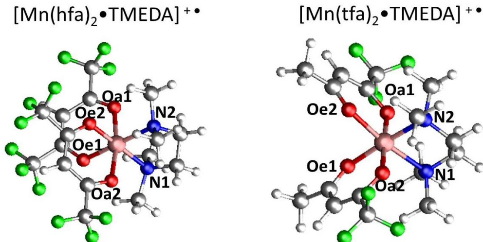
Figure 4. Calculated minimum structures of [\text{Mn}(\text{dik})_2 \cdot \text{TMEDA}]^{+\bullet} radical cations in the quintet spin state. Atom color codes as in Figure 1.
