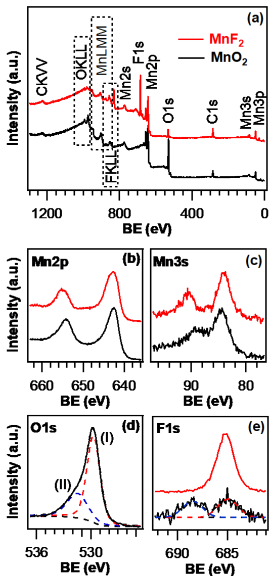
Figure 7. (a) Surface-wide-scan XPS spectra for \text{MnF}_2 and \text{MnO}_2 specimens. The detailed (b) \text{Mn}2p , (c) \text{Mn}3s , (d) \text{O}1s , and (e) \text{F}1s surface photoelectron peaks pertaining to the two samples are also reported.
