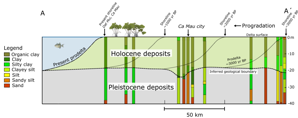
Figure 2. Lithological borelogs of the Division of Water Resources Planning and Investigation for the South (DWRPIS) of Vietnam and Division for Geological Mapping for the South (DGMS) of Vietnam along the transect A-A'. The boundary between the Holocene deposits, mainly consisting of organic clays (clays with high organic matter content), clays and silty clays and the underlying coarser and stiffer Pleistocene deposits is highlighted. The prodelta gradient is determined by profile measurements of the submarine delta front at the west side of the present VMD. The north part of the section A-A' demarcates the present boundary between the lower and the upper delta plain 28 . The lithological profile at Dat Mui has been obtained from Surface Elevation Table (SET) 29 .
