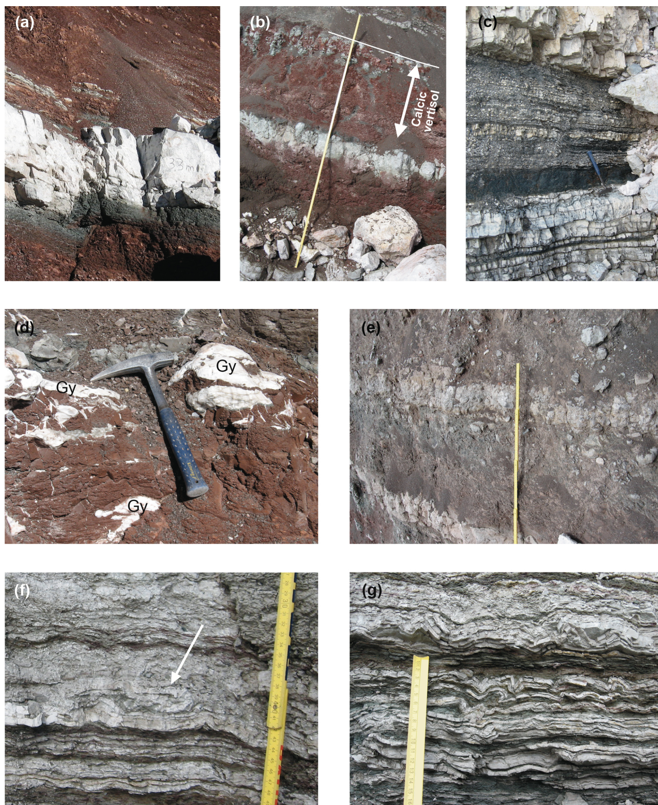
Figure 3. Outcrop images of different types of dolomite intercalated with red and grey clay of the Travenanzes Fm. at Rifugio Dibona: (a) homogeneous dolomite bed (15 cm thick; 33 m). (b) Upper part: dolomite nodules embedded in red clay, cross-cut by green-coloured cracks that are part of a calcic Vertisol (95 m). (c) Laminated dolomite (110–112 m) interbedded with grey clay. (d) Bed containing gypsum nodules (Gy), along with gypsum-filled cracks at 50 m; (e) Dolomite-cemented conglomerate bed at 75 m. (f) Laminated bed showing soft sediment deformation (106 m); an isoclinal syndimentary fold is indicated by the arrow. (g) Laminated dolomite showing folding of the laminae due to soft sediment deformation (same bed as in f).
