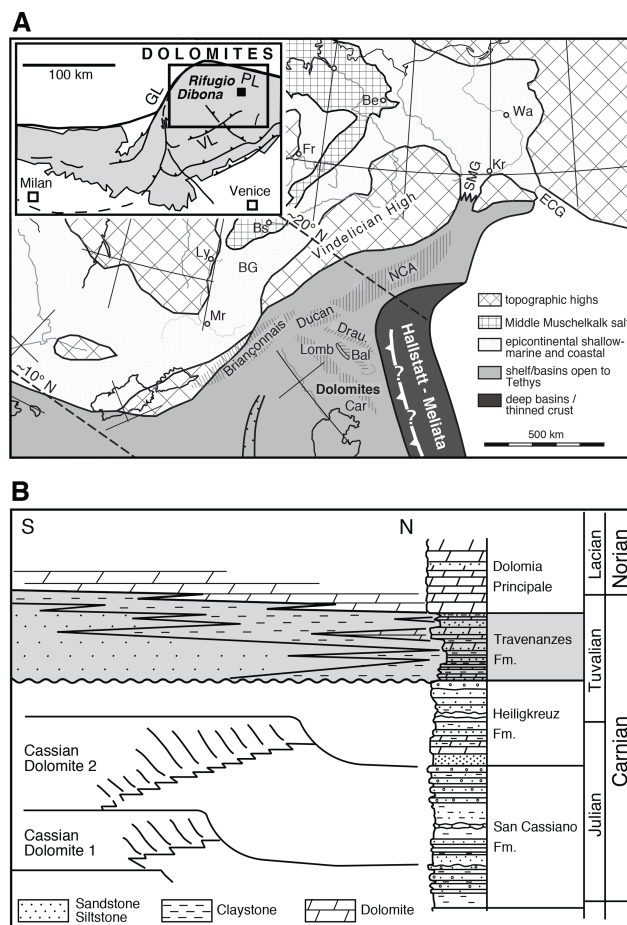
Figure 1. (a) Palaeogeographic map of southern Alpine to Germanic domains during the middle Triassic; reproduced from Brack et al. (1999; modified). Bal: Balaton; BG: Burgundy Gate; Car: Carnian Alps; ECG: eastern Carpathian Gate; Lomb: Lombardy; NCA: Northern Calcareous Alps; SMG: Silesian Moravian Gate. The following cities are indicated for orientation: Mr: Marseille; Wa: Warsaw; Kr: Kraków; Be: Berlin; Fr: Frankfurt; Ly: Lyon. Inset: tectonic map of the southern Alps (Brack et al., 1996; modified) showing the sampling location at Rifugio Dibona. GL: Giudicarie Line; PL: Pustertal Line; VL: Val Sugana Line. (b) Middle to Upper Triassic stratigraphy and distribution of facies within the Venetian Alps, showing a transition in geometries from a basin and platform topography during the lower Carnian to an extended alluvial to tidal plain in the upper Carnian. The shaded area indicates the Travenanzes Fm., showing a lateral transition in facies and a transgressive boundary with the Dolomia Principale. Compiled from Breda and Preto (2011), after De Zanche et al. (1993); modified.
