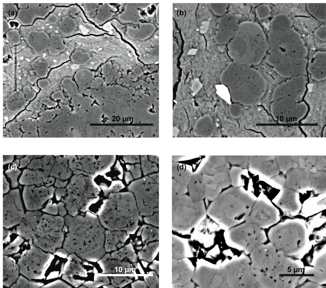
Figure 6. SEM images of dolomites in backscatter mode showing different types of crystal shape: (a) spheroidal growth of dolomite (darker areas) in clay layers (brighter areas; sample TZ14-9d; 95 m); (b) close-up of (a); (c, d) dolomite crystals showing a porous interior and homogeneous syntaxial cement rims (c: sample TZ14-12; 90 m; d: sample TZ14-9d; 95 m).
