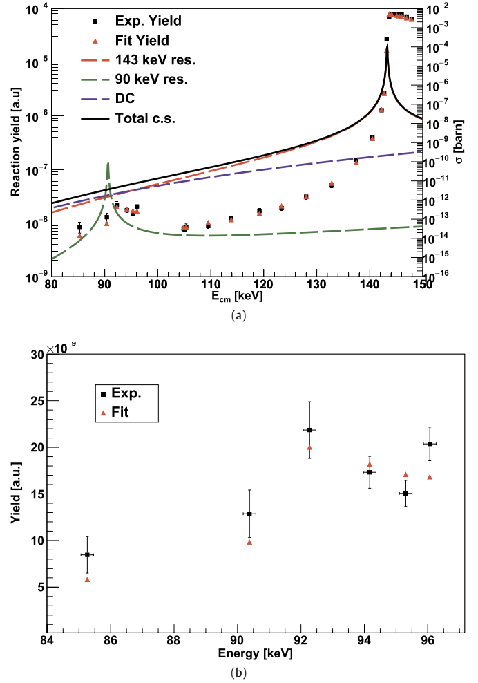
Fig. 2. (a) Experimental yield and fitted cross section of ^{18}\text{O}(p, \gamma)^{19}\text{F} . The total cross section and the direct and resonant components are shown as lines. The left axis refers to the yield points, the right one to the cross sections (lines). Displayed in the inset is a zoom into the low energy resonance region. (b) Experimental data vs. fit results in the low-energy region.
