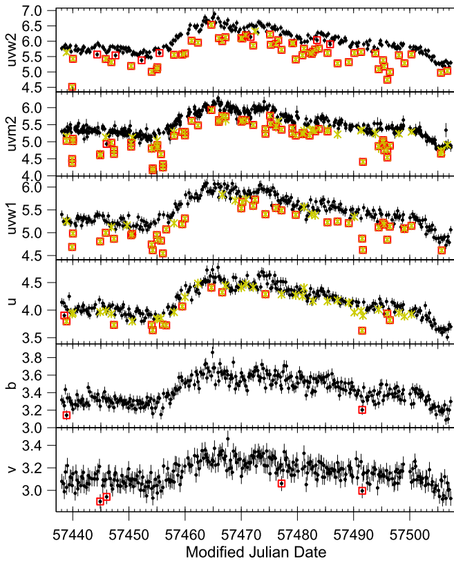
Figure 1. NGC 4151 light curves before filtering. Y-axis fluxes are given in units of 10^{-14} \text{ erg cm}^{-2} \text{ s}^{-1} \text{ Å}^{-1} . Points flagged as dropouts are shown as red boxes. These points are also shown in red in Figure 2, where they are used to define “bad detector regions.” Points in the four shortest-wavelength bands that fell in those bad regions (yellow in Figure 2) are also shown in yellow in this figure. Finally, the black points are the remaining good data that passed our filtering.
