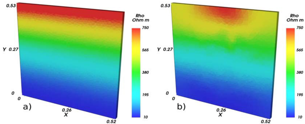
Fig. 5 ERT true resistivity model (a) and inverted model (b) for the 8-source numerical experiment with quadratic resistivity distribution
