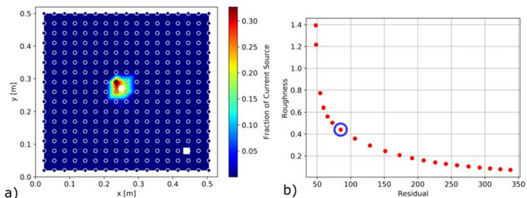
Fig. 3 Numerical synthetic test. a) The synthetic test evaluates the iCSD capability to locate a current point source (white dot). The white circles represent the VRTE and the white square the return electrode. The source of current was centered between four VRTE to highlight the distribution of the current density. While the
