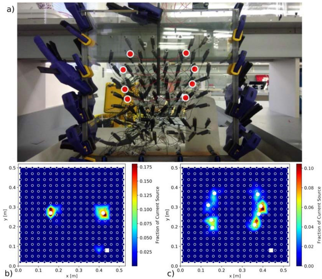
Fig. 4 Laboratory tests. a) Rhizotron filled with water for the tests with metallic wires. The plastic insulation of the metallic wires avoided the current leakage, which occurred only where the insulation was removed (eight red dots). This test simulated a complex and root-like structure, with the current leaking at the tips. b) result of iCSD test with two metallic sources in water. c) result of iCSD
