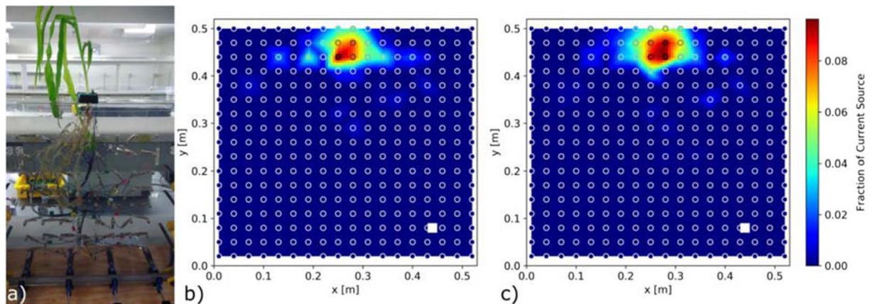
Fig. 8 Hydroponic experiments with a maize plant. a) Position of the plant and roots, with the root crown approximately 3 cm below the water surface. b-c) CSD obtained from the iCSD: the current
