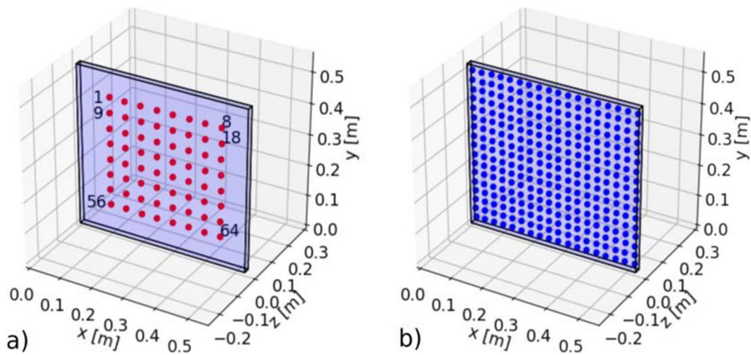
Fig. 2 Rhizotron setup. Dimensions are 53x52x2 cm. a) the 64 silver/silver chloride electrodes were distributed to maximize both ERT and MALM data quality and coverage, thus enhancing the
