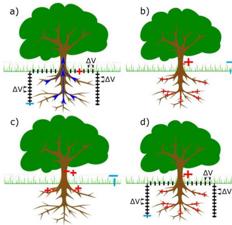
Fig. 1 Electrical approaches for estimating root geometry and functioning. The figures describe the physical conceptualization and electrode positions for the ERT (a), BIA (b, c), and iCSD (d) methods. The red cross and the blue dash are the current injection electrodes. The black dashes are the potential electrodes, used to image the electric potential field (ERT and iCSD). a) The ERT method characterizes the RWU through its impact on the soil moisture content and, consequently, on the soil resistivity. b) The
