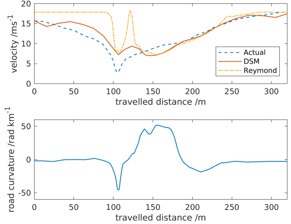
Fig. 5: Example of cornering testcase (Test C4)
