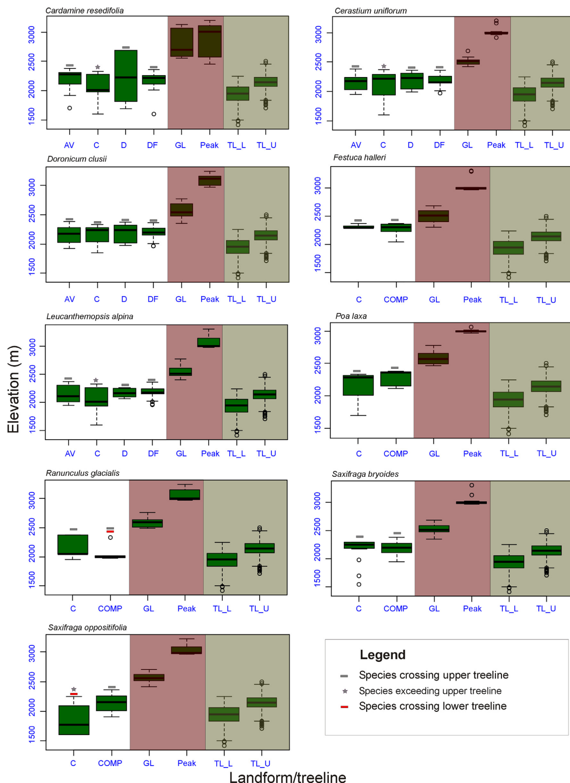
Fig. 5. Mean elevation of alpine species typical of peak areas at different landform slope deposits or landform units and compared with the mean elevation of treelines. Circles represent outliers. Brown background colour highlights the elevation range of the species in their typical alpine habitat. Green background colour highlights the elevation range of the upper and lower treelines. Legend: AV = Avalanche deposits; C = Channels; D = Rock/debris fall deposits; DF = Debris flows deposits; GL = Recent glacial deposits; Peak = Peak area; U_TL = Upper treeline; L_TL = Lower treeline. (For interpretation of the references to colour in this figure legend, the reader is referred to the web version of this article.)
