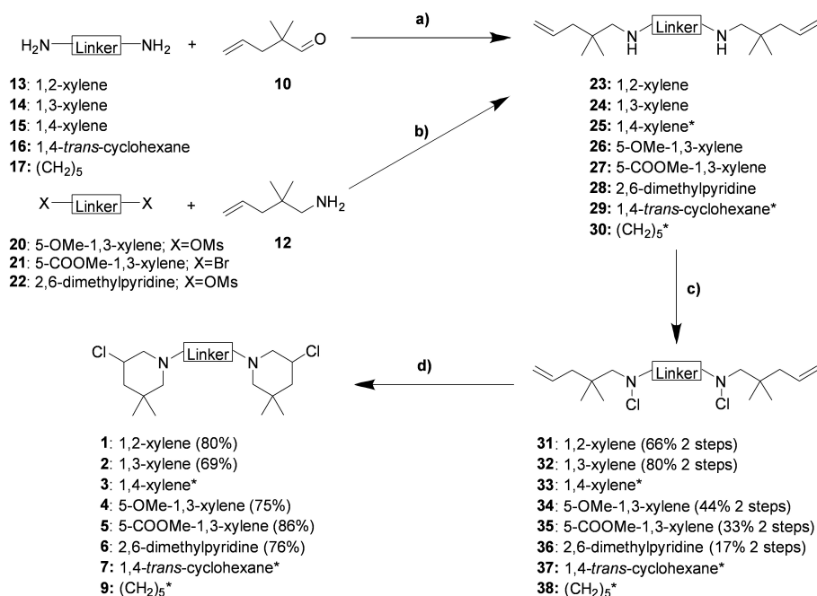
Scheme 1. Synthesis of bis-3-chloropiperidines 1–6. a) NaBH(OAc) 3 , AcOH, dry CH 2 Cl 2 , 0 °C to RT, 16–18 h; b) NaH, dry THF, 0 °C to RT, 20–22 h; c) NCS, dry CH 2 Cl 2 , 0 °C to RT, 2.5–3 h; d) TBAI (cat.), dry CHCl 3 , 60 °C (oil bath temperature), 2–2.5 h (inseparable diastereomeric mixture). *The synthesis of compounds 3, 7 and 9 as well as their corresponding precursors has been described elsewhere. [4b]
