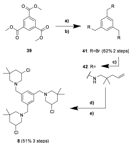
Scheme 2. Synthesis of tris-3-chloropiperidine 8. a) LAH, dry THF, 0 °C to RT to reflux, 18 h; b) PBr 3 , dry Et 2 O, 0 °C to RT, 24 h; c) 2,2-dimethylpent-4-en-1-amine 12, dry CH 2 Cl 2 , 0 °C to RT, 68 h; d) NCS, dry CH 2 Cl 2 , 0 °C to RT, 2.5 h; e) TBAI (cat.), dry CHCl 3 , reflux, 4 h.
