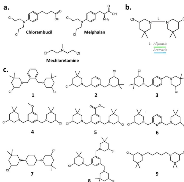
Figure 1. a) Chemical structure of chlorambucil, melfalan and mechlorethamine. b) General structure of B–CePs. Different connecting linkers (L) are schematized with different colors. c) Chemical structures of the analyzed 3-chloropiperidines.
