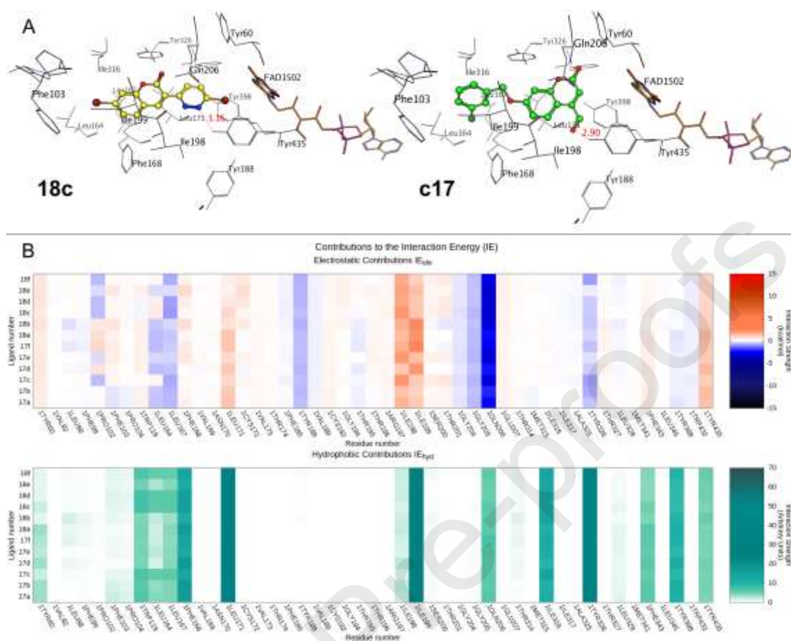
Figure 7. Panel A, the pose of 18c (in yellow) is compared to the crystallographic conformation of c17 (PDB ID: 2v60, in green). In Panel B it is reported the contribution of each residue to the interaction energy focusing to the electrostatic and hydrophobic interactions. The strength of the IE_{ele} and IE_{hyd} contribution is color-coded according to their strength computed by MOE scoring function.
