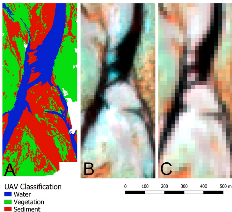
FIGURE 4. Example of (A) UAV-derived label data and corresponding Sentinel-2 imagery at (B) 10 m of spatial resolution and (C) 20 m of spatial resolution. [Colour figure can be viewed at wileyonlinelibrary.com ]
