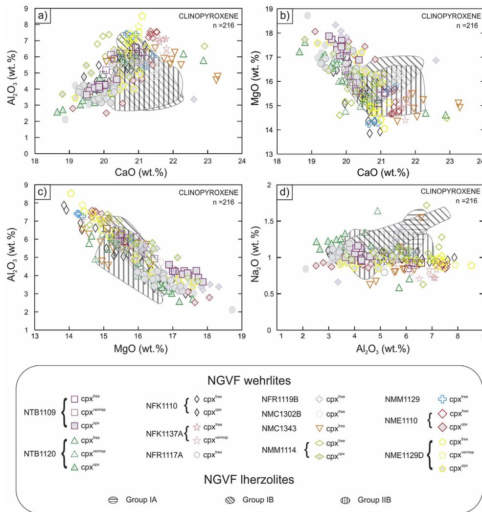
Fig. 11. Major element compositions of wehrlitic clinopyroxenes appearing in different textural positions compared to distinct NGVF lherzolites of Liptai et al. (2017). (a) CaO vs. \text{Al}_2\text{O}_3 ; (b) CaO vs. MgO; (c) MgO vs. \text{Al}_2\text{O}_3 ; (d) \text{Al}_2\text{O}_3 vs. \text{Na}_2\text{O} . (cpx free —vermicular spinel and orthopyroxene free clinopyroxenes; cpx verm —clinopyroxenes hosting vermicular spinel; cpx opx —clinopyroxenes hosting orthopyroxene).
