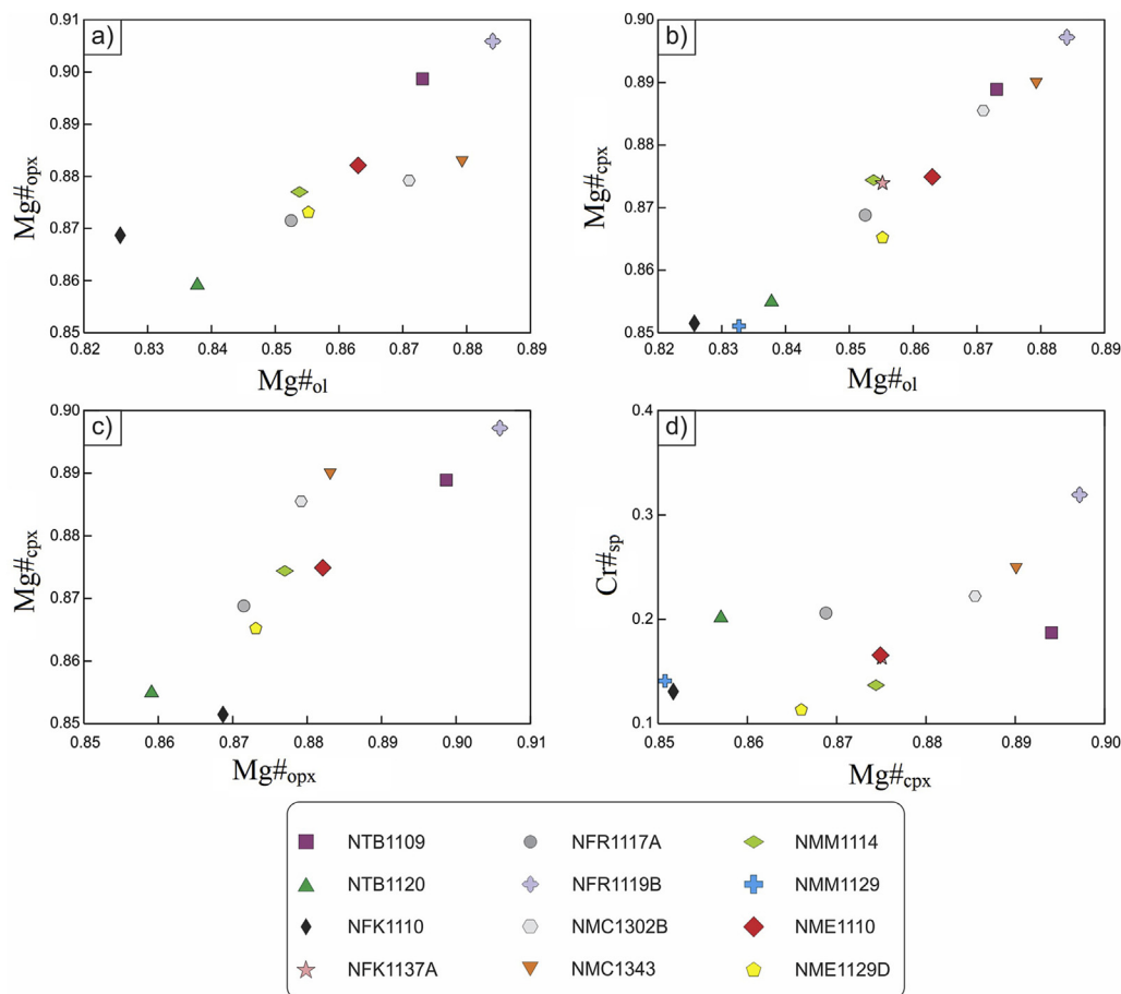
Fig. 12. Relationships between (a) Mg\#_{ol} vs. Mg\#_{opx} , (b) Mg\#_{ol} vs. Mg\#_{cpx} , (c) Mg\#_{opx} vs. Mg\#_{cpx} , (d) Mg\#_{cpx} vs. Cr\#_{sp} . Note that the Cr\# of the vermicular spinels was excluded in evaluating the averages.
