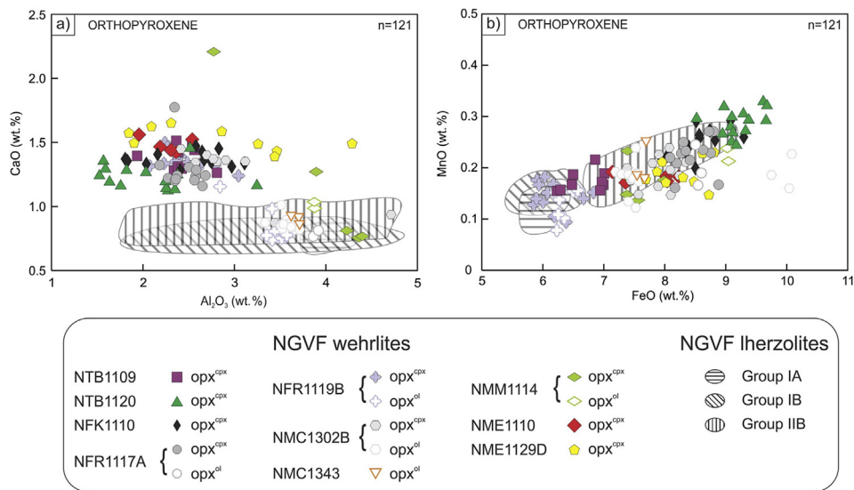
Fig. 5. (a) Al 2 O 3 vs. CaO and (b) FeO vs. MnO relationships in orthopyroxene with respect to their textural position (opx cpx – orthopyroxenes hosted by clinopyroxenes; opx ol – orthopyroxenes hosted by olivines). The different NGVF lherzolite groups are from Liptai et al. (2017).
