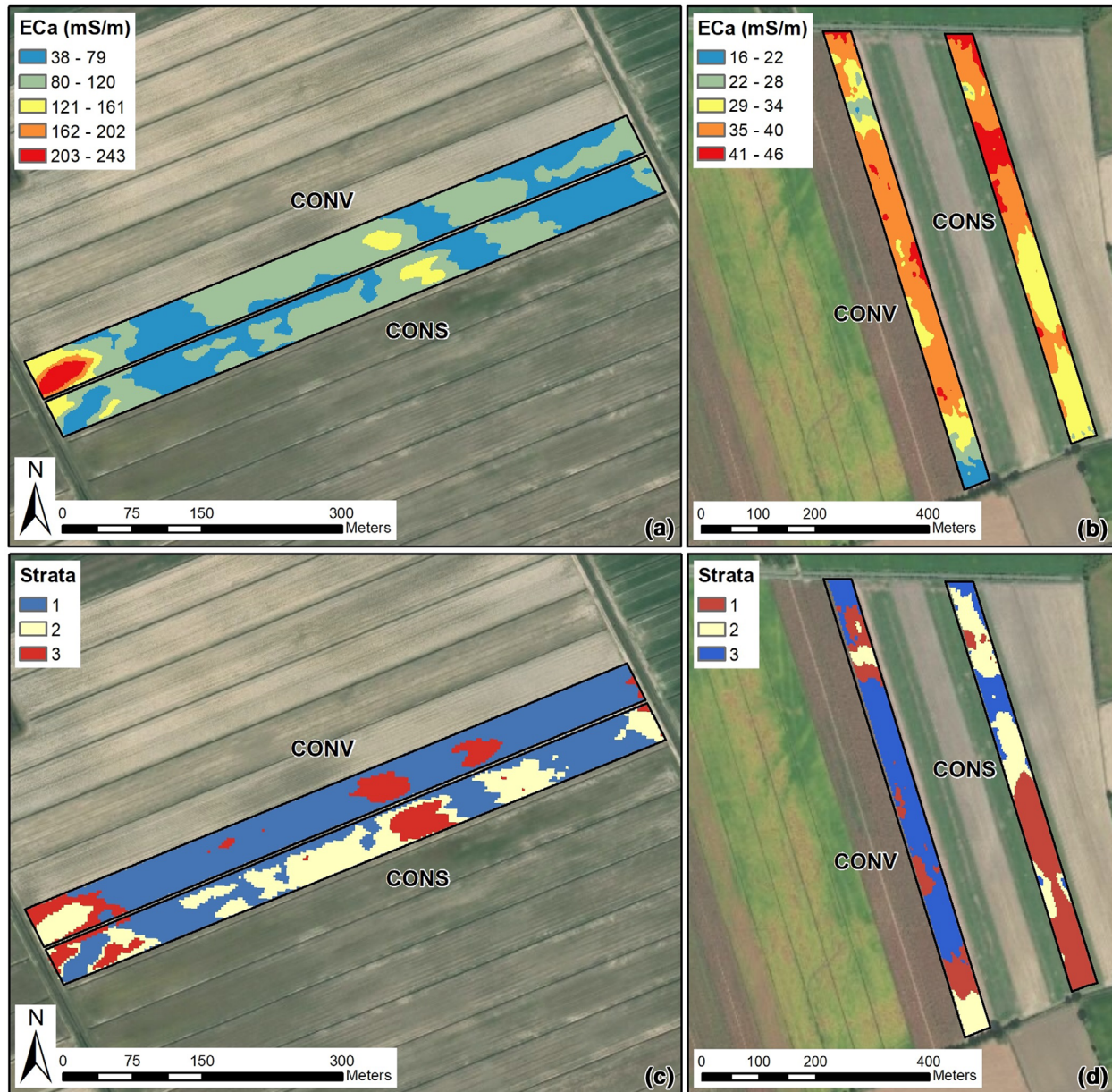
FIGURE 4 Ordinary kriging of soil apparent electrical conductivity ( EC_a ) at 0- to 90-cm depth through vertical coplanar configuration at (a) F1 and (b) F2. Panels c and d report EC_a -based stratification by k -means clustering. CONS, conservation agriculture; CONV, conventional tillage
