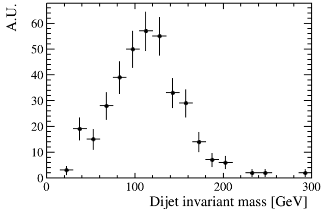
Figure 15. The di-jet invariant mass of truth-matched b -jets in H \rightarrow b\bar{b} full-simulated events at \sqrt{s} = 1.5 TeV.
