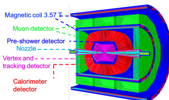
Figure 3. Schematic view of the detector, with each component identified by the label.
