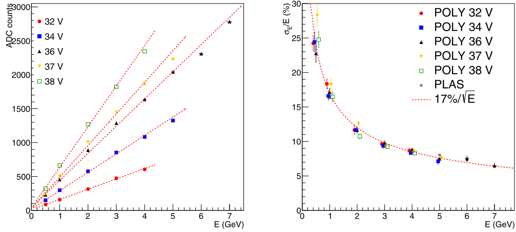
Fig. 9. Linearity with electron energy (left) and electron energy resolution (right) for POLY at different values of the SiPM applied voltage.
