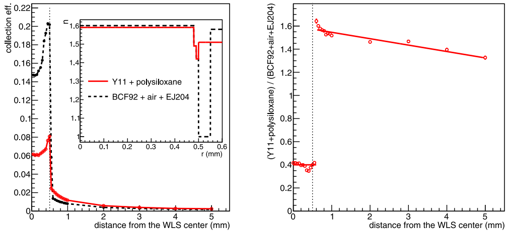
Fig. 2. GEANT4 optical simulation results. Left: Collection efficiency as a function of the distance from the WLS center for the Y11 + polysiloxane (solid red) and the BCF92 + air + EJ204 (dashed black) setups. Right: ratio of the collection efficiencies for the two setups. The dotted vertical line represents the boundary of the WLS fiber. The inset in the left plot shows the refractive index from the fiber center for the polysiloxane (solid red) and the plastic scintillator (dashed black) configurations. The refractive index of the outer part of Y11 WLS is, from the core to the outer cladding, 1.59, 1.49, 1.42 (1.05, 1.19, 1.43 g/cm 3 ) while that of polysiloxane is 1.51 (1.01 g/cm 3 ). The refractive index of EJ-204 is 1.58 (1.023 g/cm 3 ) while that of BCF-92 is 1.60, 1.49, 1.42 (1.05 g/cm 3 density for the core). The vertical line represents the boundary of the WLS fiber.
