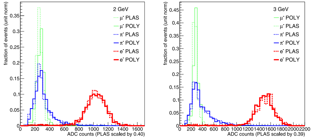
Fig. 8. Distributions of the pulse heights for POLY (solid) and PLAS (dashed) at a SiPM bias voltage of 36 V for different particle populations (thicker red line for e^- , medium thick blue for \pi^- and thinner green for \mu^- ) as selected using the Cherenkov counters pair. Left and right plots refer to a beam energy of 2 and 3 GeV respectively.
