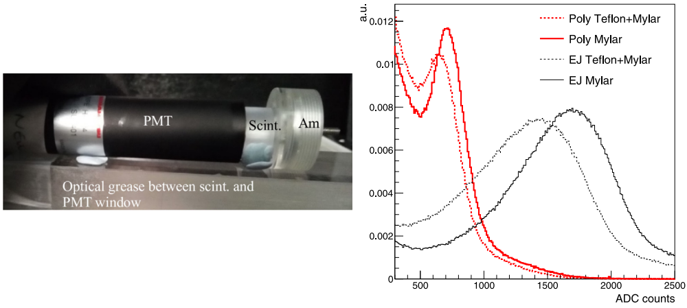
Fig. 1. Comparison of light yields with sources. Left: The setup with the Am source, the scintillator cylinder and the photomultiplier. Right: pulse spectra for the Eljen scintillator (thin black) and the polysiloxane one (thick red). Dashed (solid) histograms are obtained with wrapping 1 (2), respectively, see text.
