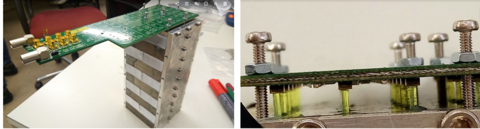
Fig. 5. WLS-SiPM coupling. Left: a single module with the PCB installed in the back plane. Right: a close-up lateral view of the PCB with fixing bolts. The Y11 WLS fibers touching the SiPM are visible and could be individually inspected.
