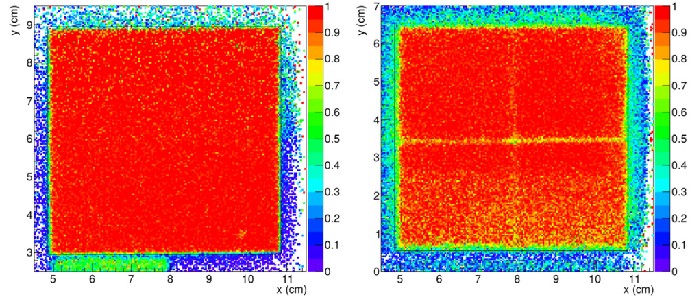
Fig. 10. Efficiency map for the PLAS (left) and POLY (right) upstream UCM with a 20 ADC counts threshold (color version online).
