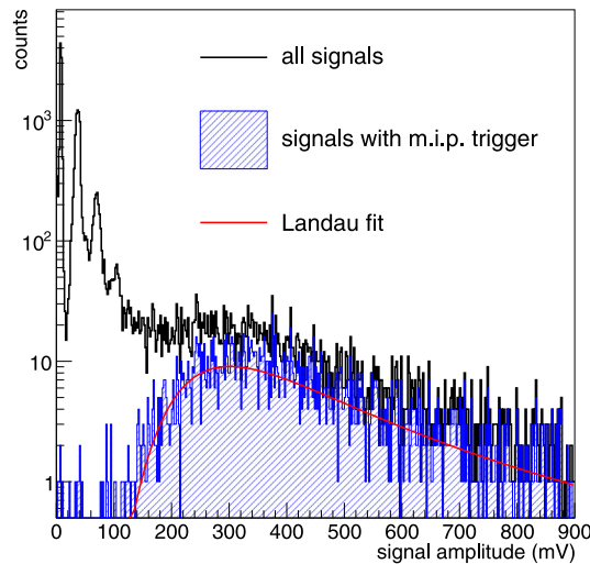
Fig. 15. Left: the amplifier connected directly on the SiPM PCB for the measurement of single photo-electron peaks of the central SiPM of the UCM. Right: the spectra of the digitized signal amplitude in the acquisition time window for POLY at a bias voltage of 38 V. The black histogram shows the distribution for all acquired waveforms while the blue filled one (with a Landau function fit superimposed) is for the subsample of single-cluster events in which the particle enters the fiducial volume of the calorimeter. (For interpretation of the references to color in this figure legend, the reader is referred to the web version of this article.)
