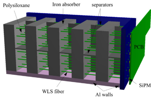
Fig. 3. Polysiloxane prototype. Left: annotated sketch of a single module (4 UCMs). Right: a picture of the three calorimeter modules (12 UCMs).
