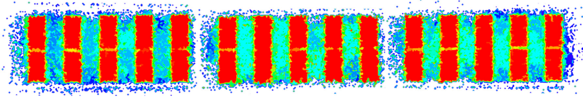
Fig. 13. Lateral efficiency maps with a 10 ADC threshold for the three modules. The free surface of the liquid polysiloxane is down in this figure (color version online).
