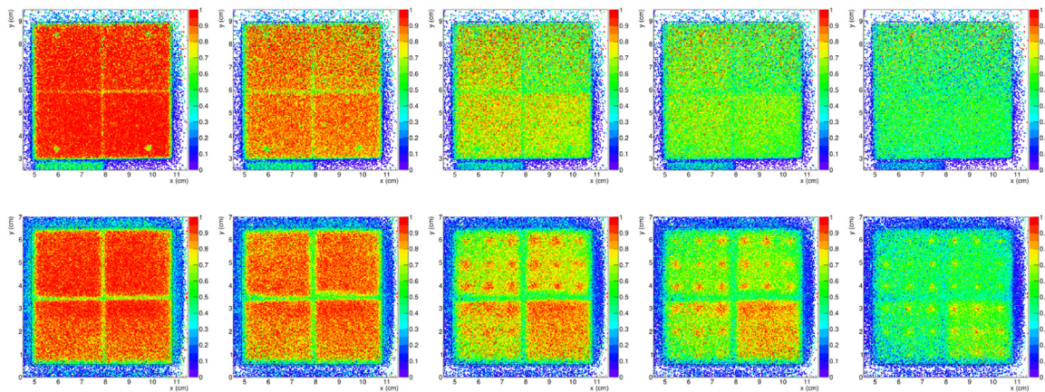
Fig. 11. Efficiency maps for increasing thresholds from left to right for the most upstream module using all particle types. The upper row refers to PLAS the lower one to POLY (color version online).
