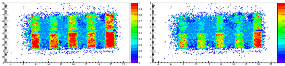
Fig. 14. Lateral efficiency maps at different thresholds of 30 (left) and 35 (right) ADC counts for the upstream module as an example (color version online).
