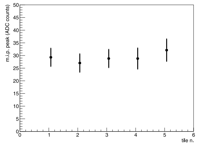
Fig. 12. Light yield of the scintillator tiles. Tiles are ordered from 1 to 5 according to their position along the beam direction. Markers represent the means of the most probable values for Landau fits of mip tracks for each tile position in the UCMs, while their spreads is shown by the error bar.
