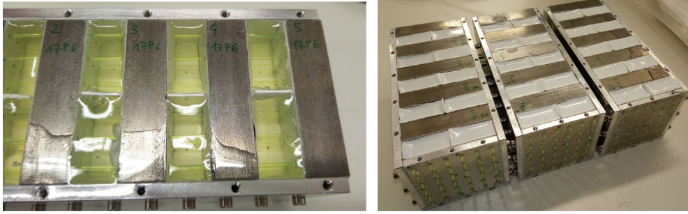
Fig. 4. Polysiloxane prototype. Left: close up of scintillator compartments. Right: the full prototype with a white diffuser on the surface face.
