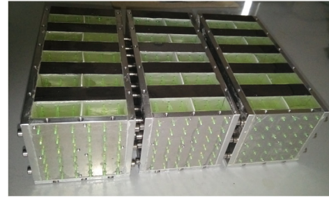
Fig. 3. Polysiloxane prototype. Left: annotated sketch of a single module (4 UCMs). Right: a picture of the three calorimeter modules (12 UCMs).
