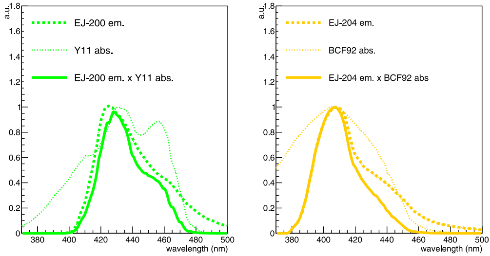
Fig. 7. Right: spectral matching between BCF92 fibers and EJ-204 scintillator, equivalent to the PLAS setup. Left: spectral matching between Y11 fibers and EJ-200, corresponding to the POLY setup (EJ-200 emission is very similar to the used polysiloxane-based scintillator).
