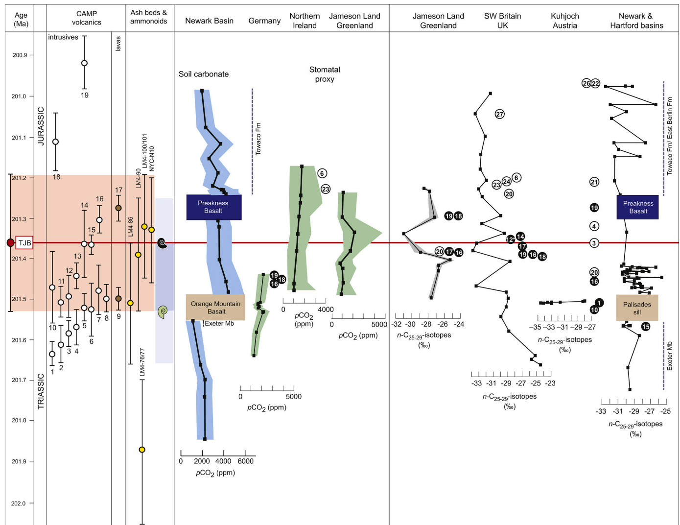
Fig. 10. Correlation and comparison of pCO_2 -records from pedogenic carbonate in the Newark Basin (Schaller et al., 2011; Schaller et al., 2016) and from plant fossil cuticles (stomatal index) from Germany (Bonis et al., 2010a), Northern Ireland and Jameson Land, Greenland (Steinthorsdottir et al., 2011), with C-isotopes from C_{25-29} n-alkanes from Greenland (Williford et al., 2014), SW Britain in UK (Whiteside et al., 2010), Kuhjoch in Austria (Ruhl et al., 2011) and the Newark and Hartford basins in eastern USA (Whiteside et al., 2010). Please note that there is a difference in scale of the Exeter Member, between the soil carbonate record (Schaller et al., 2011, 2016) and the n-alkane record (Whiteside et al., 2010). A list of all the biostratigraphic events can be found on Fig. 7.
