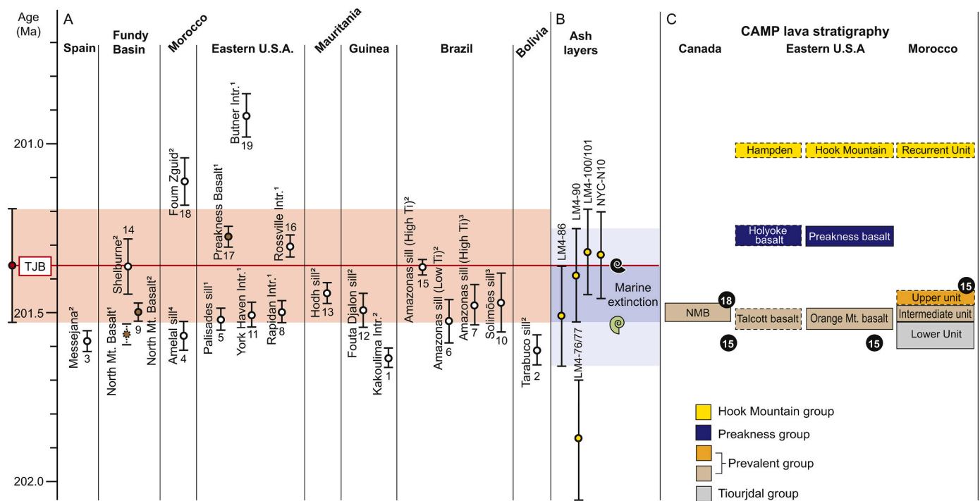
Fig. 2. A) Geochronology of CAMP intrusions (white circles) and lava flows (brown circles), after 1 Blackburn et al. (2013) , 2 Davies et al. (2017) , 3 Heimdal et al. (2018) ; 4 Marzoli et al. (2019) . Ages of intrusions and lava flows, numbered 1–19, appear on Figs. 3–11. B) Geochronology of ash beds (yellow circles) from the sedimentary ammonoid bearing successions in Nevada ( Schoene et al., 2010 ) and Pucara Basin, Peru ( Schoene et al., 2010 ; Wotzlaw et al., 2014 ). Green ammonoid symbol represents the last occurrence (LO) of Choristoceras crickmayi and the black ammonoid symbol represents the first occurrence (FO) of Psiloceras spelae ( Schoene et al., 2010 ; Wotzlaw et al., 2014 ). The latter defines the Triassic–Jurassic boundary (TJB), marked as a red line, estimated to 201.36 \pm 0.17 Ma by Wotzlaw et al. (2014) ; pink field represents the estimated error. Dark blue field marks the marine extinction interval, defined as the interval between the LO of C. crickmayi or C. marshi and the FO of P. spelae ( Schoene et al., 2010 ; Hillebrandt et al., 2013 ). The light blue field shows the approximate maximum duration of the mass extinction interval, based on U-Pb ages of ash beds LM4-86 and LM4-90 ( Schoene et al., 2010 ; Wotzlaw et al., 2014 ). C) Schematic stratigraphy of CAMP lavas, mainly after Marzoli et al. (2011) . Hitherto undated units are marked by stippled boxes. Thickness (i.e. as a proxy for apparent duration) of volcanic units is only indicative. Black circles with numbers represent last occurrences of Triassic pollen taxa (shown on Fig. 3): 15) Patinasporites densus , and 18) Lunatisporites rhaeticus , after Cirilli et al. (2009) and Panfili et al. (2019) . A complete list of all the biostratigraphic events used on Figs. 2–10 can be found on Fig. 7.
