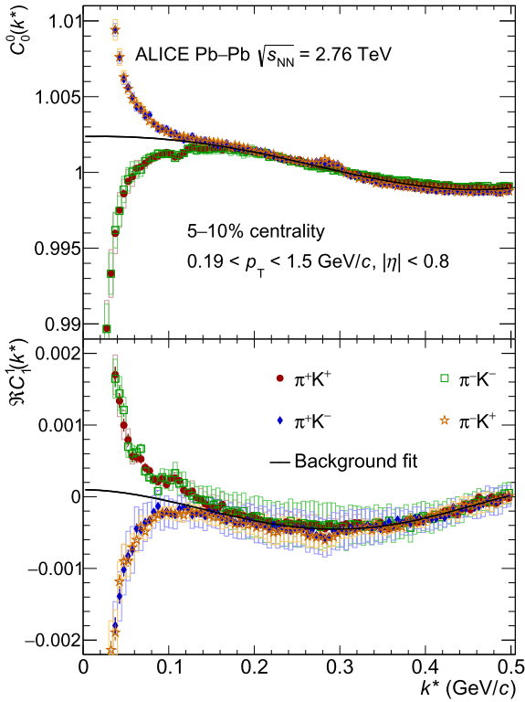
Fig. 2. The C_0^0 (top panel) and \text{Re}[C_1^1] (bottom panel) components of the pion-kaon correlation functions in the 5–10% centrality class showing the non-femtoscopic background in the spherical-harmonic representation, positive field polarity. The background fit corresponds to a 6th order polynomial function common for all charge combinations. The two structures visible in the correlation function at 0.11 GeV/c and at 0.29 GeV/c correspond to the remaining effect from track merging and the K^* resonance, respectively. The statistical and systematic uncertainties are shown as vertical bars and boxes, respectively.
