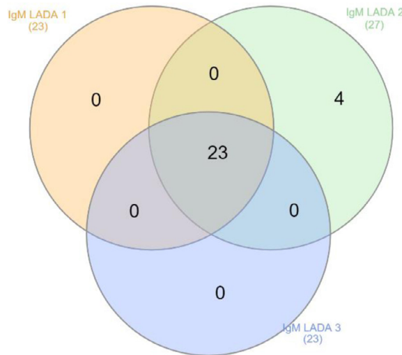
Fig. 3. Venn diagram. Venn diagram of serum cross-reactivity for IgMs positive to peptides Ac-hGAD65(250-273)-NH 2 (1), Ac-hGAD67(258-281)-NH 2 (2), and Ac-CVB4P2C(28-50)-NH 2 (3) in LADA patients
