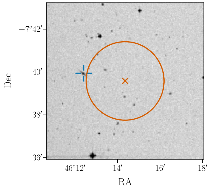
Figure 5. Overlay of the estimated 90% Swift/BAT error radius for GRB 190610A (orange circle) on the sky. A galaxy at around 165 Mpc (Dálya et al. 2018) compatible with this localization is indicated by the blue crosshair.
