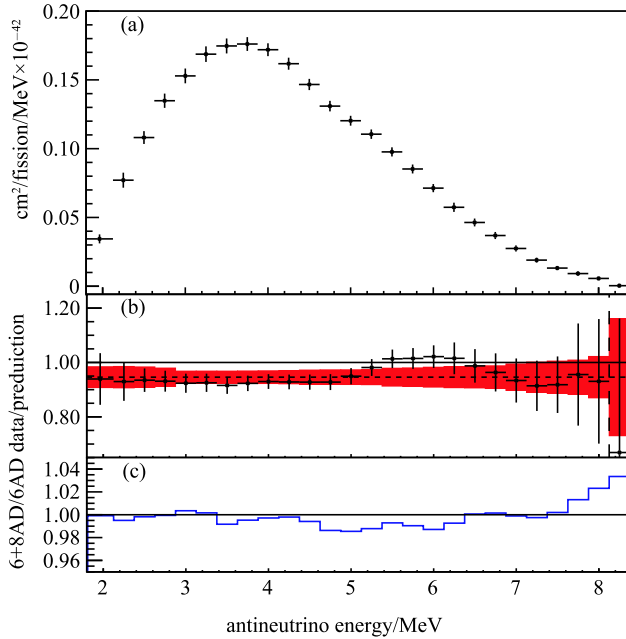
Fig. 28. (color online) (a) The antineutrino spectrum weighted by the IBD cross section. The last bin is integrated up to 12 MeV. (b) Ratio of the extracted reactor antineutrino spectrum to the Huber+Mueller prediction. The error bars of the data points are the square-roots of the diagonal elements of the antineutrino spectrum covariance matrix. The solid red band represents the square-roots of the diagonal elements of the prediction covariance matrix, including both reactor and Huber+Mueller model uncertainties. (c) the ratio of the spectra from the 6+8 AD periods used in this analysis and the 6 AD period used in the previous analysis [29].
