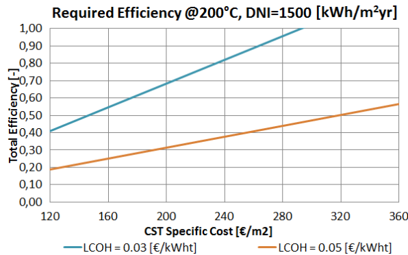
Fig. 9. Required CSLFC efficiency as a function of specific cost, @200°C, DNI= 1500 kWh/m 2 yr
