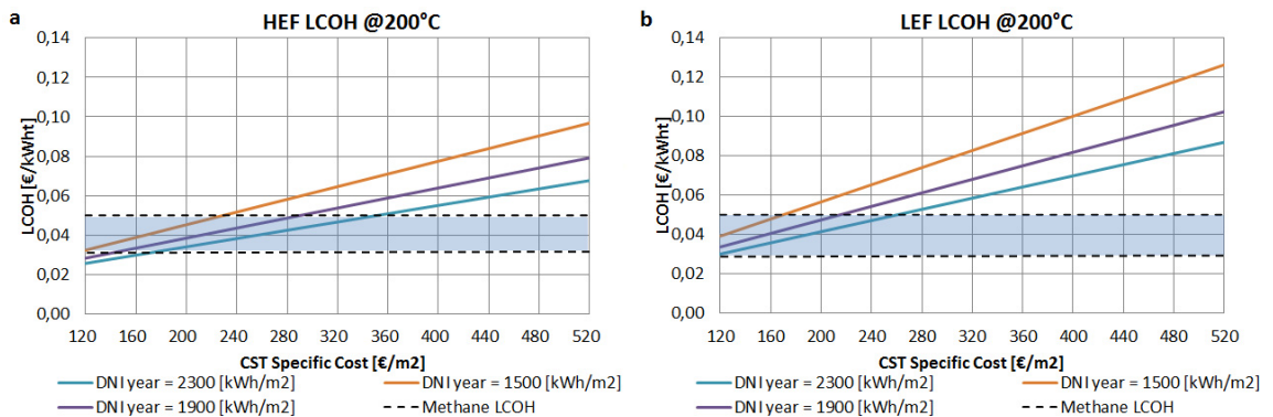
Fig. 6. LCOH at T = 200°C at latitude of 35°N for (a) HEF systems; (b) LEF systems
