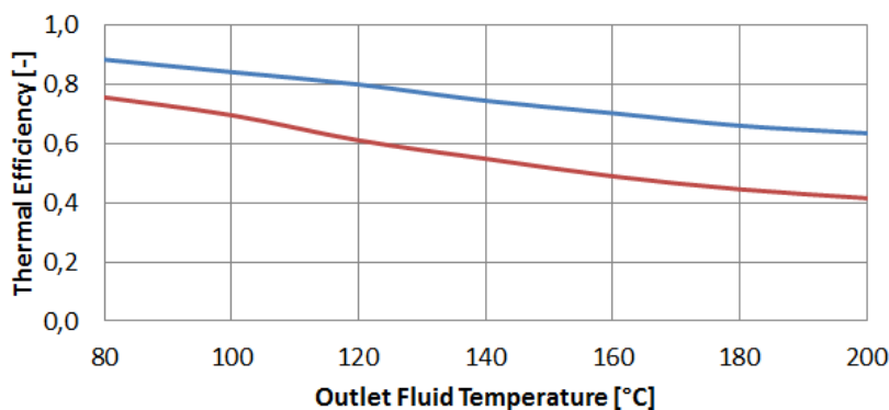
Fig. 4. Thermal Efficiency for HEF and LEF systems
