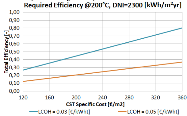
Fig. 7. Required CSLFC efficiency as a function of specific cost, @200°C, DNI= 2300 kWh/m 2 yr
