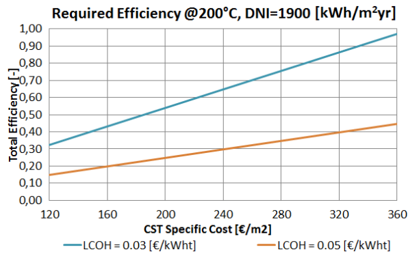
Fig. 8. Required CSLFC efficiency as a function of specific cost, @200°C, DNI= 1900 kWh/m 2 yr
