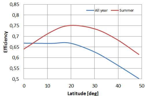
Fig. 3. Optical efficiency for different latitudes.
