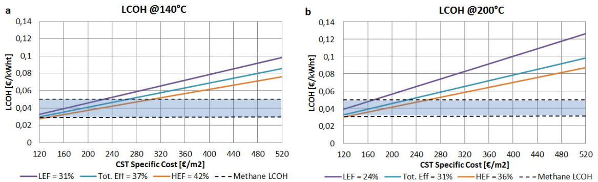
Fig. 5. (a) LCOH at T = 140°C; (b) LCOH at T = 200°C
