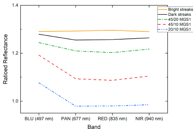
Fig. 10. Ratiod reflectance averages for bright (orange solid line) and dark slope streaks (black solid line), and MoHIS spectrometer MGS-1 CaSSIS convolved spectral ratios for selected particle size fractions. A similar ratio feature can be observed from PAN to BLU for both lab and CaSSIS dark slope streak spectra, which indicates a possible particle size effect. Slope streak spectra taken from Fig. 5. Y axis offset for clarity.
