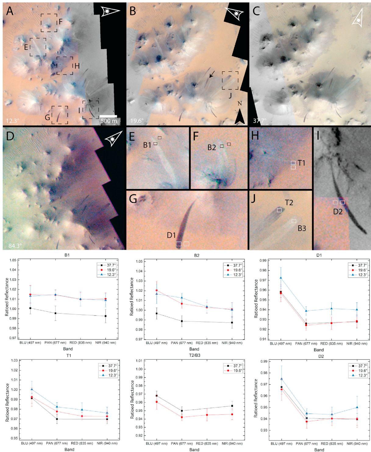
Fig. 7. (A–D) CaSSIS multi-angular observations of various slope streaks for site S16. (E–J) ROI close ups selected for relative photometry (B1, B2, T1, D1 and D2). No photometric analysis was performed on (D), it is only shown here to display the importance of high SNR and good atmospheric conditions in identifying slope streaks. CaSSIS multi-angular ratioed reflectance plots for the terminus of bright (B1 and B2), dark (D1 and D2) and transitioning (T1) streaks at site S16. Ratio plot (T2/B3) of transitioning talus (T2) and bright talus (B3) streak also provided. A general brightening with decreasing phase is observed on all slope streaks. The dark streaks (D1 and D2) and the transitioning streak (T1) show a sharp decrease in ratio at the CaSSIS BLU band (497 nm). A similar effect can be seen in transitioning (T2) and bright streak (B3) termini ratio plot (T2/B3). Phase angles are shown on the bottom left (A–D).
