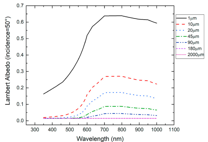
Fig. 11. Modeled Lambert albedo reflectance curves for different grain sizes. The model was run for particle size fractions similar to those analyzed in the lab. The plot illustrates that the smallest particles <10 μm exhibit the largest increase in albedo. The incidence angle was set to equal 50° in order to analyze the reflectance dependence on particle size, unrelated to opposition surge phenomena. Based on optical constants derived from CRISM/OMEGA measurements (Wolff et al., 2009).
