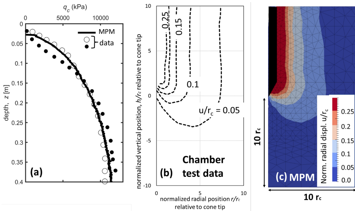
Figure 6 cone penetration in sand [28] (a) cone resistance; (b) normalized radial displacement in chamber test and (c) in MPM. Cone radius is r_c .
