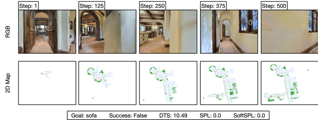
Figure 5. A failed episode with the ANS* variant. The agent explored the environment for 500 steps without finding any Sofa occurrence. Green pixels on the map are the obstacles, light blue pixels are explored areas, and the blue point is the goal position.
