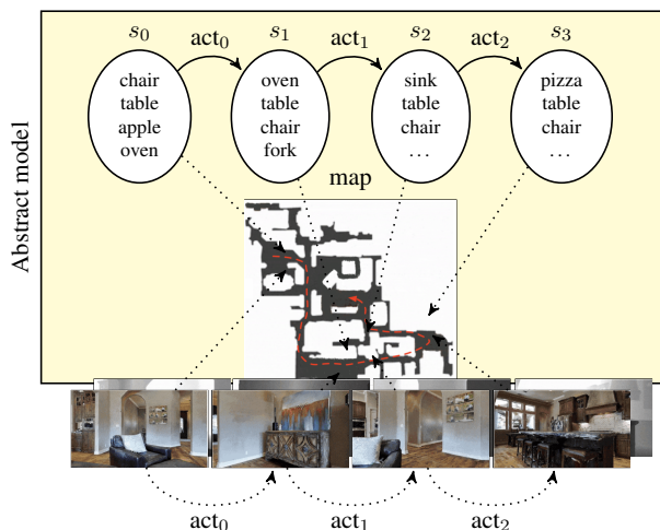
Figure 1. During its navigation in a complex 3D scenario, an agent incrementally acquires knowledge about the environment by storing rich semantic information in an Abstract Model. For instance, when the robot is in s_0 , chair and table are visible; by performing act_0 , other objects become visible, thus the Abstract Model is updated to s_1 . Our work shows how knowledge can be incrementally learned and effectively reused over time.
