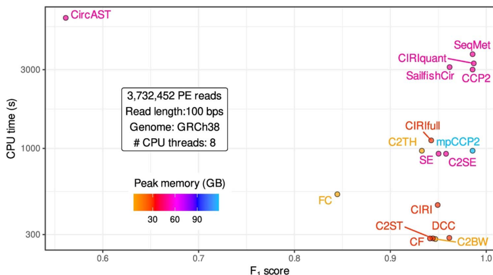
Figure 6. Computation time and memory requirements of circRNA detection methods. F 1 -scores of 14 circRNA detection pipelines compared to their computing time in seconds (s) and peak random access memory (in GigaBytes) required to process ~3.7 million paired-end (PE) reads of 100 bp length, mapped to the human genome (GRCh38) and using eight CPU threads for each tool. Plus, one hypothetical pipeline running sequentially the seven methods used in CirComPara2 (SeqMet) and CirComPara2 set with maximal parallelization settings (mpCCP2) allowing to run up to seven tasks in parallel, for peak usage of 56 CPU threads in total.
