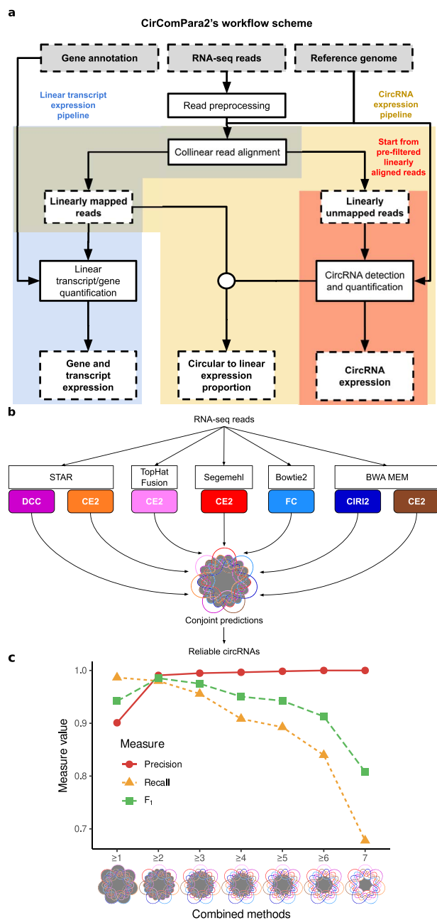
Figure 2. The CirComPara2 workflow and approach. A , Boxes with dashed contour indicate input and output data; boxes with solid-line contour indicate computing tasks; the circular connector indicates merging data. Background colours highlight the different pipeline branches (linear transcript analysis in blue, full circRNA analysis in yellow and strict circRNA analysis in red). B , A detail of the CirComPara2 strategy ('CircRNA detection and quantification' box in a ) showing the embedded circRNA detection methods (coloured rounded corner boxes) with the respective chimeric read aligners (white boxes). The central Venn diagram represents the optimized combination of method prediction intersections implemented by CirComPara2 with circRNAs conjointly detected by two or more methods (grey filled intersections) retained as default. Method abbreviations as in Figure 1 . C , Precision (red), recall (yellow) and F 1 -score (green) for different numbers of methods that conjointly identified the circRNAs: \geq 1 indicates that at least one method identified the circRNAs, or, in other words, it represents the union of all single methods predictions; \geq 2 indicates the circRNAs conjointly predicted by two or more methods; \geq 3 indicates the circRNAs commonly identified by any combination set of at least three methods; similar is for the larger number of methods sharing the predictions. The '7' indicates circRNAs commonly predicted by all the methods. The grey-filled parts in Venn diagrams show the intersections considered by the conjoint method combinations.
