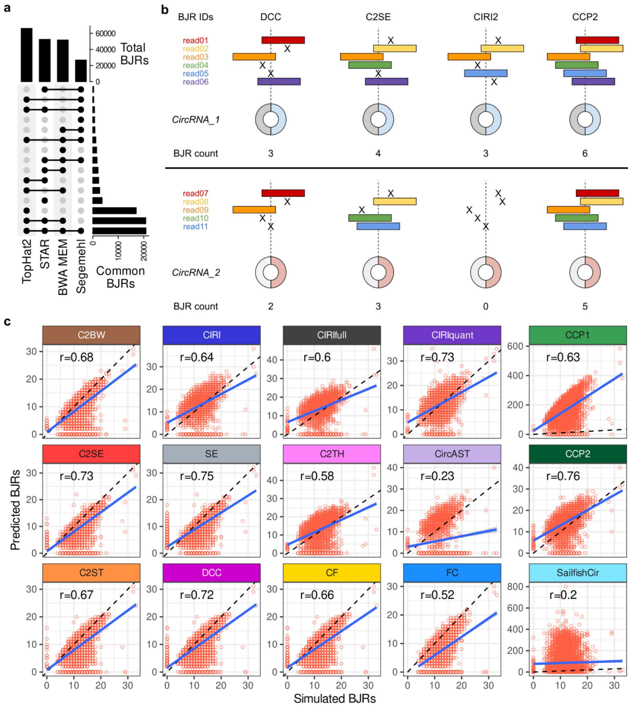
Figure 5. CircRNA expression estimates from CirComPara2. A , The overlap between the different sets of the back-splice junction reads (BJRs) identified by four chimeric aligners (BWA-MEM, Segemehl, STAR and TopHat-Fusion/TopHat2). B , The CirComPara2 BJR count approach: the upper panel shows the non-redundant BJR count of CirComPara2 (CCP2) compared to other methods (for simplicity, only three methods are displayed), which is based on unique BJR identifiers (BJR IDs); the lower panel highlights how CCP2 can preserve the information even when no BJR is in common between circRNA detection methods. C , The estimated circRNA expression in BJR compared to the true expression from the simulated data set. The Pearson correlation coefficient ( r ) values are reported in the boxes. CIRIquant, CircAST and Sailfish-cir were inputted with the circRNAs predicted by CirComPara2.
