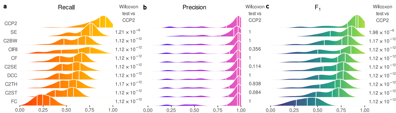
Figure 4. Performance of circRNA detection methods on the real RNA-seq data set. Results of the analysis on the 71 pairs of samples of the real RNA-seq data set. Density plots of (A) recall, (B) precision and (C) F_1 -score; distribution quartiles are indicated by white vertical lines. On the right-hand side of each plot, the Bonferroni adjusted P-values of Wilcoxon paired tests contrasting each method with CirComPara2. Methods' abbreviations as in Figure 1; CCP2: CirComPara2.
